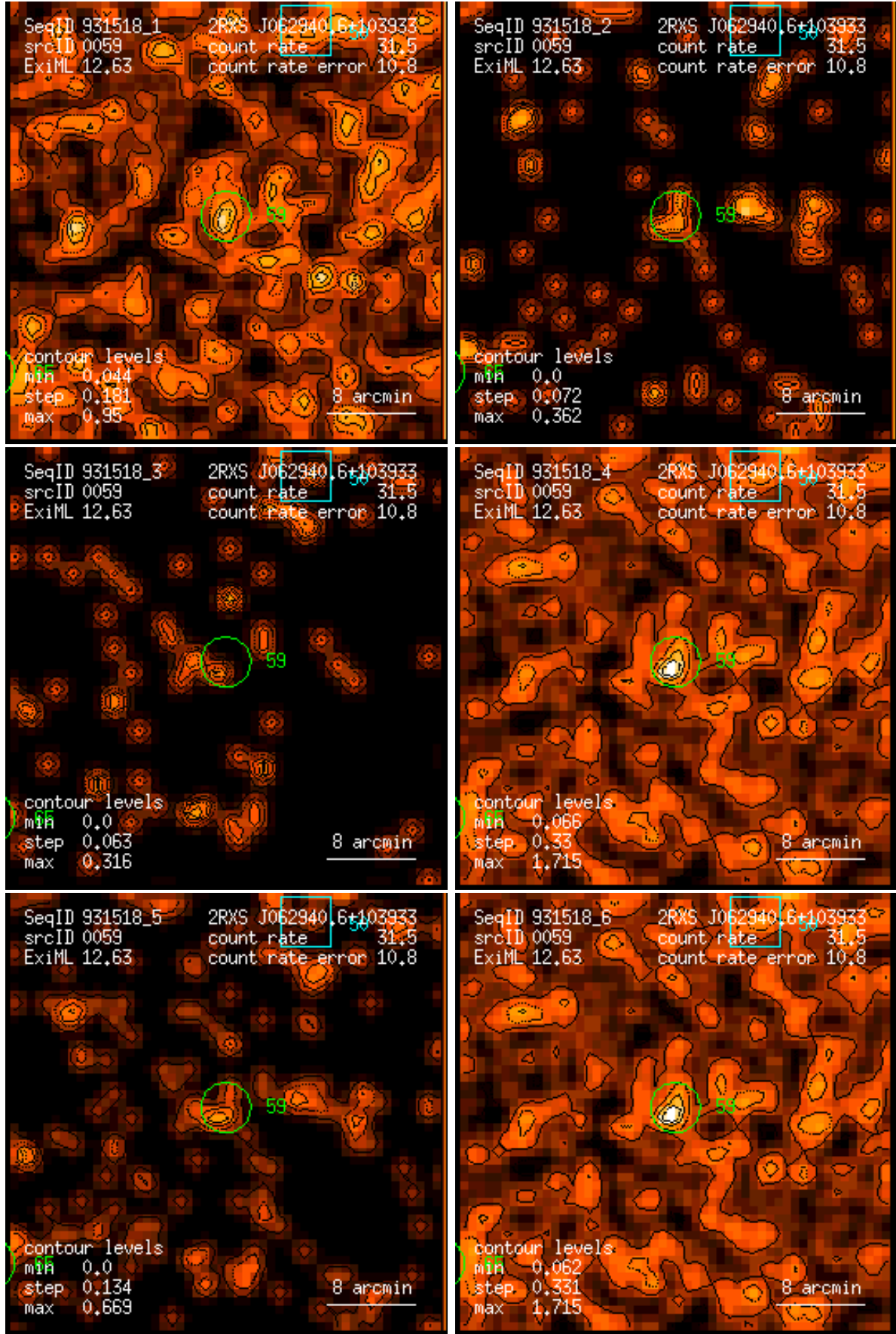
Figure 59: RASS 931518: detection 0059: band rate images, Gaussian filter: (1) PSPC channels 11 – 41, (2) 52 – 90, (3) 91 – 201, (4) 11 – 235, (5) 52 – 201, (6) 11 – 201. Broad band rates in counts/ks. Band rate contour levels in counts/ks/arcmin 2 .
