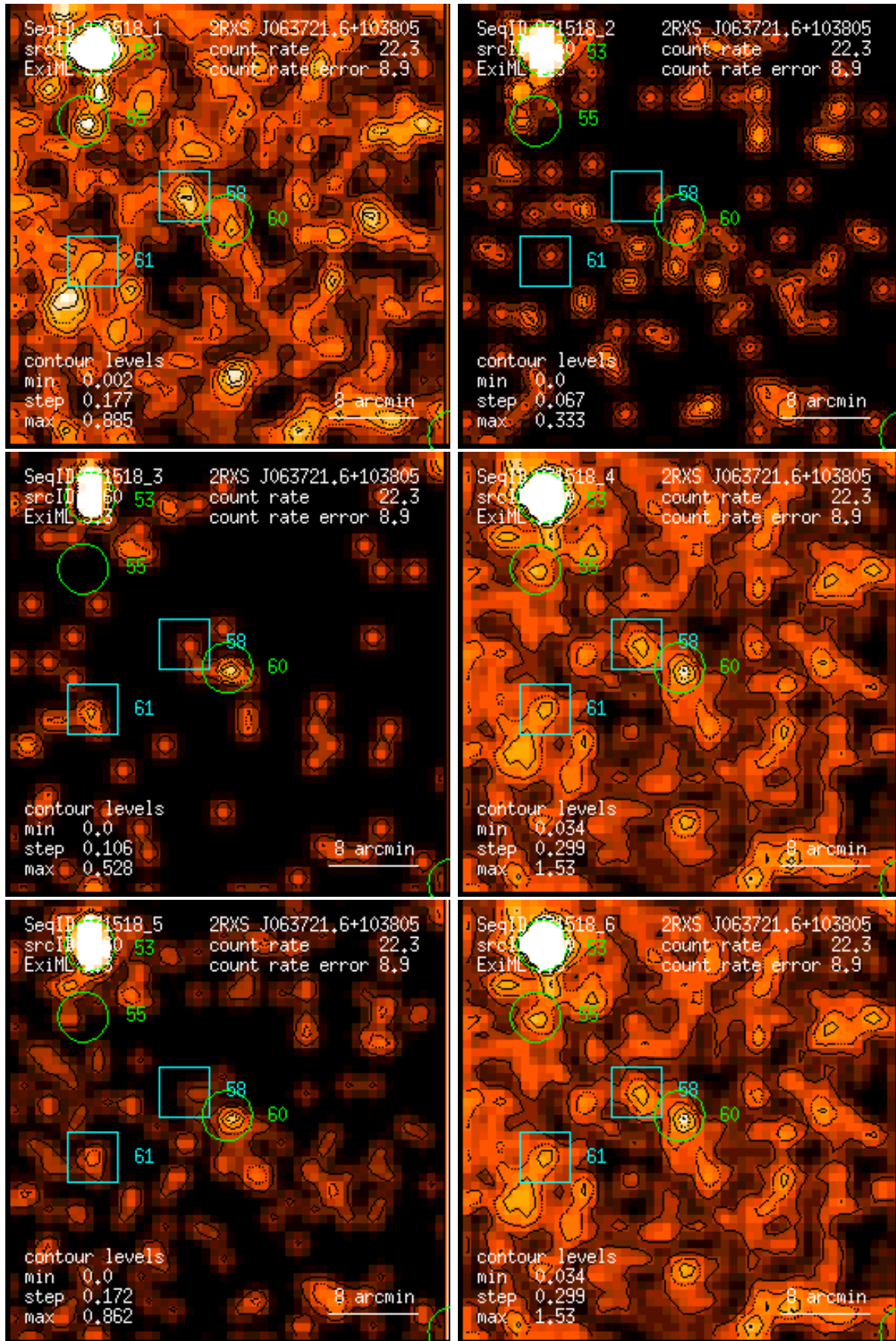
Figure 60: RASS 931518: detection 0060: band rate images, Gaussian filter: (1) PSPC channels 11 – 41, (2) 52 – 90, (3) 91 – 201, (4) 11 – 235, (5) 52 – 201, (6) 11 – 201. Broad band rates in counts/ks. Band rate contour levels in counts/ks/arcmin 2 .
