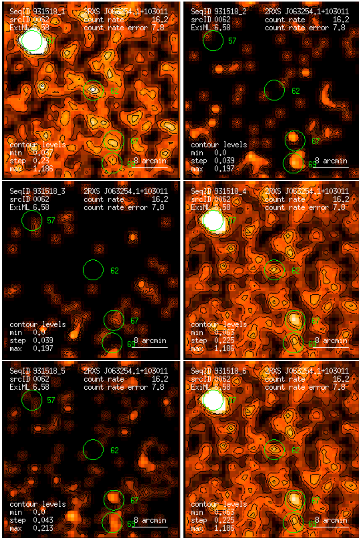
Figure 62: RASS 931518: detection 0062: band rate images, Gaussian filter: (1) PSPC channels 11 – 41, (2) 52 – 90, (3) 91 – 201, (4) 11 – 235, (5) 52 – 201, (6) 11 – 201. Broad band rates in counts/ks. Band rate contour levels in counts/ks/arcmin 2 .
