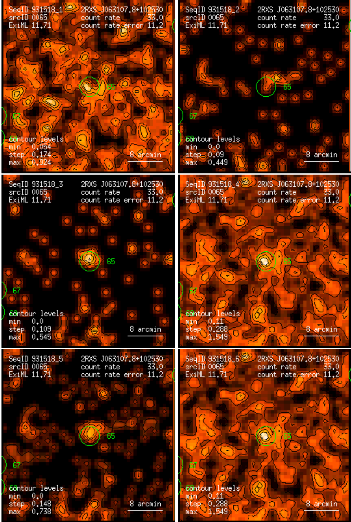
Figure 65: RASS 931518: detection 0065: band rate images, Gaussian filter: (1) PSPC channels 11 – 41, (2) 52 – 90, (3) 91 – 201, (4) 11 – 235, (5) 52 – 201, (6) 11 – 201. Broad band rates in counts/ks. Band rate contour levels in counts/ks/arcmin 2 .
