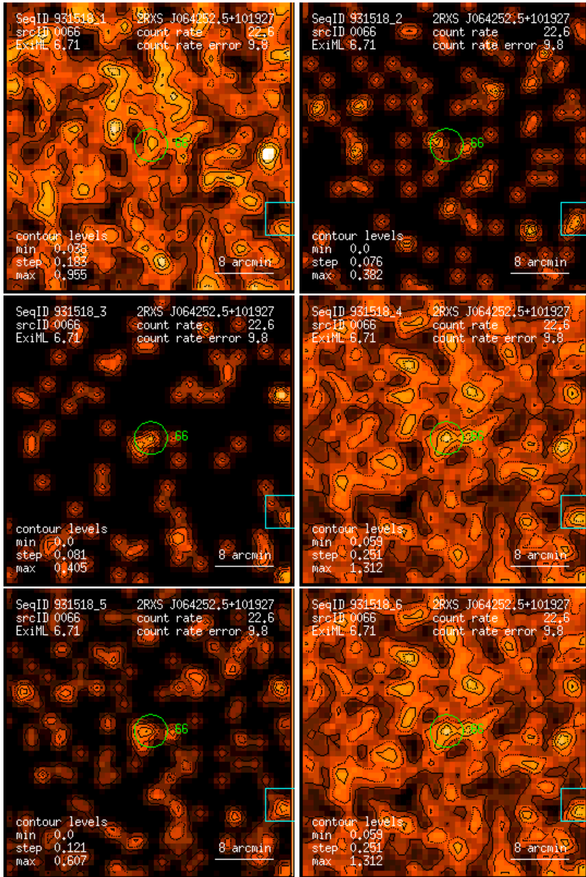
Figure 66: RASS 931518: detection 0066: band rate images, Gaussian filter: (1) PSPC channels 11 – 41, (2) 52 – 90, (3) 91 – 201, (4) 11 – 235, (5) 52 – 201, (6) 11 – 201. Broad band rates in counts/ks. Band rate contour levels in counts/ks/arcmin 2 .
