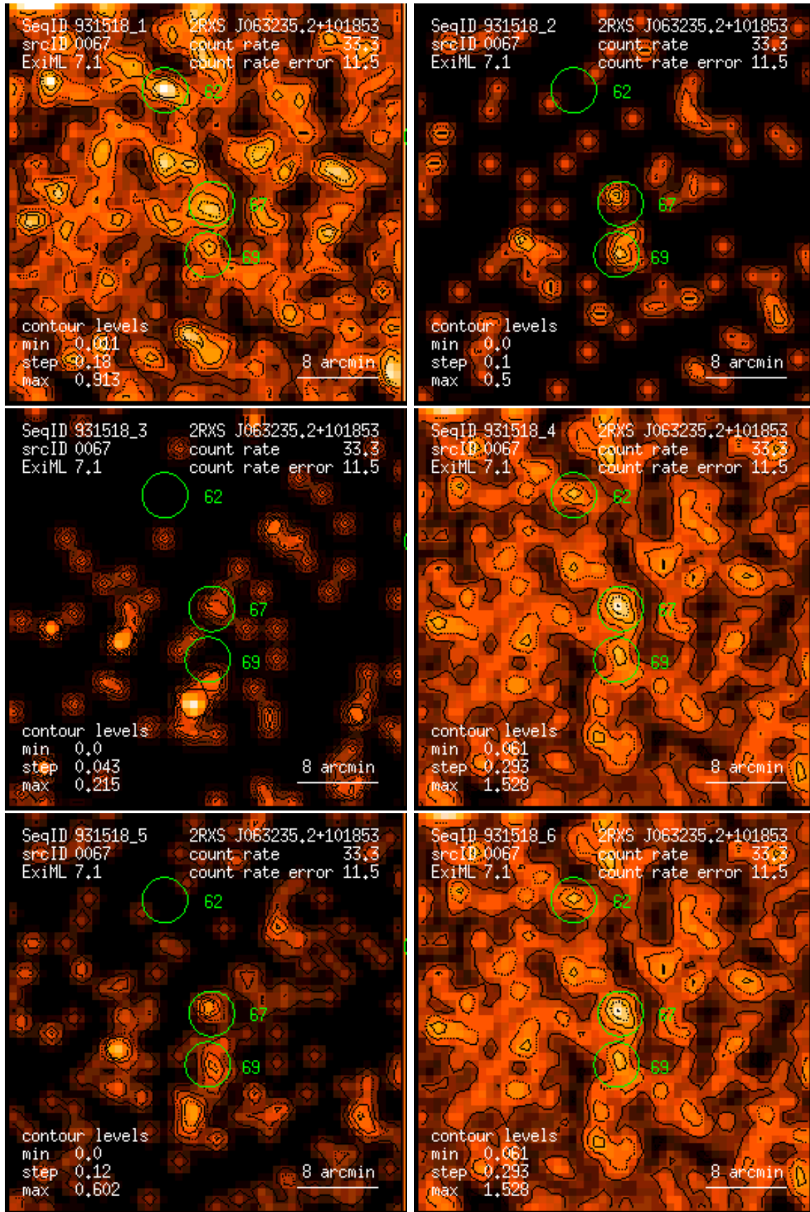
Figure 67: RASS 931518: detection 0067: band rate images, Gaussian filter: (1) PSPC channels 11 – 41, (2) 52 – 90, (3) 91 – 201, (4) 11 – 235, (5) 52 – 201, (6) 11 – 201. Broad band rates in counts/ks. Band rate contour levels in counts/ks/arcmin 2 .
