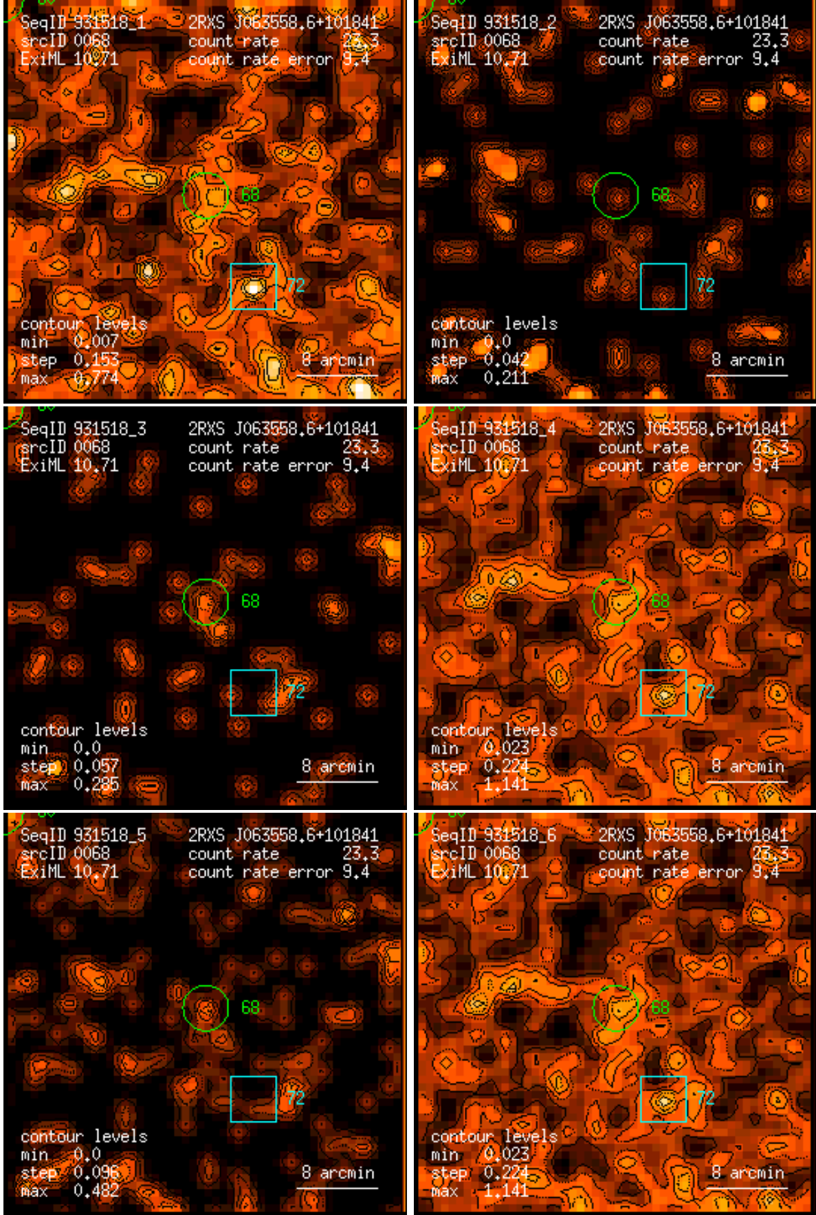
Figure 68: RASS 931518: detection 0068: band rate images, Gaussian filter: (1) PSPC channels 11 – 41, (2) 52 – 90, (3) 91 – 201, (4) 11 – 235, (5) 52 – 201, (6) 11 – 201. Broad band rates in counts/ks. Band rate contour levels in counts/ks/arcmin 2 .
