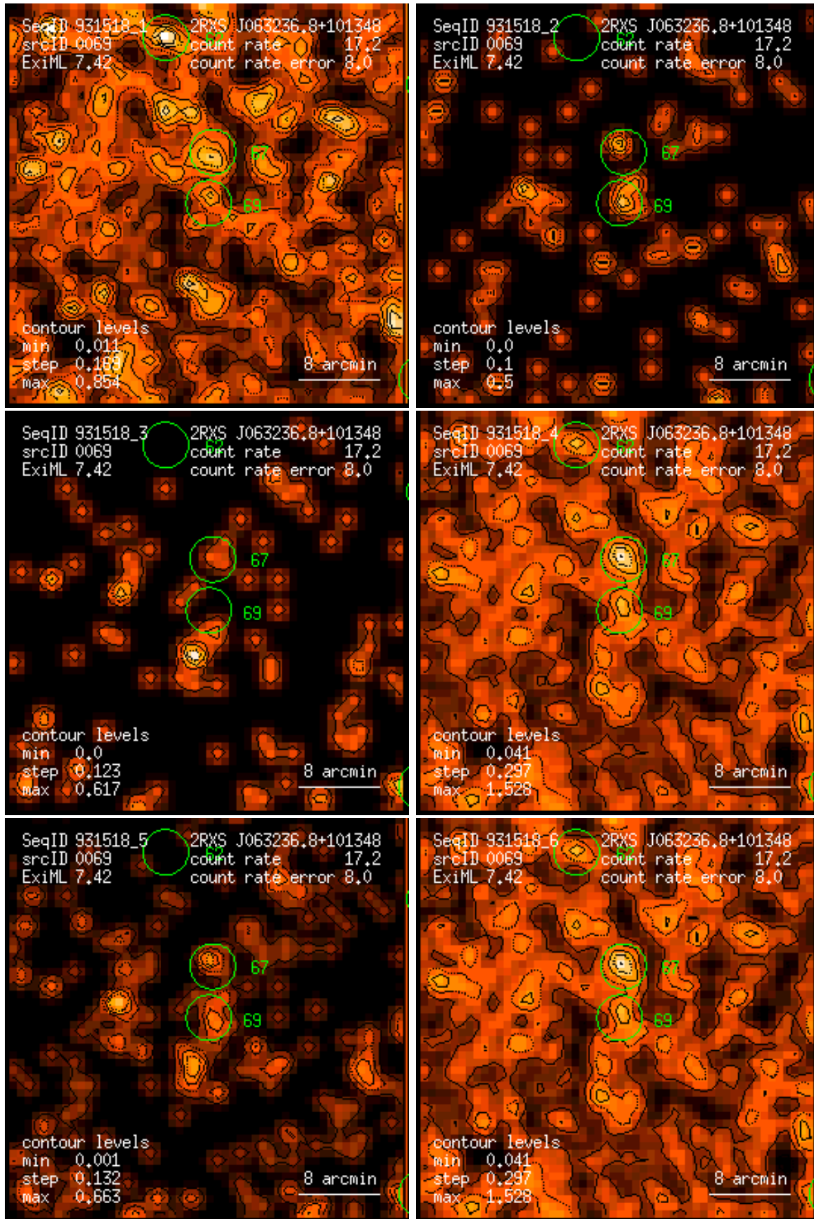
Figure 69: RASS 931518: detection 0069: band rate images, Gaussian filter: (1) PSPC channels 11 – 41, (2) 52 – 90, (3) 91 – 201, (4) 11 – 235, (5) 52 – 201, (6) 11 – 201. Broad band rates in counts/ks. Band rate contour levels in counts/ks/arcmin 2 .
