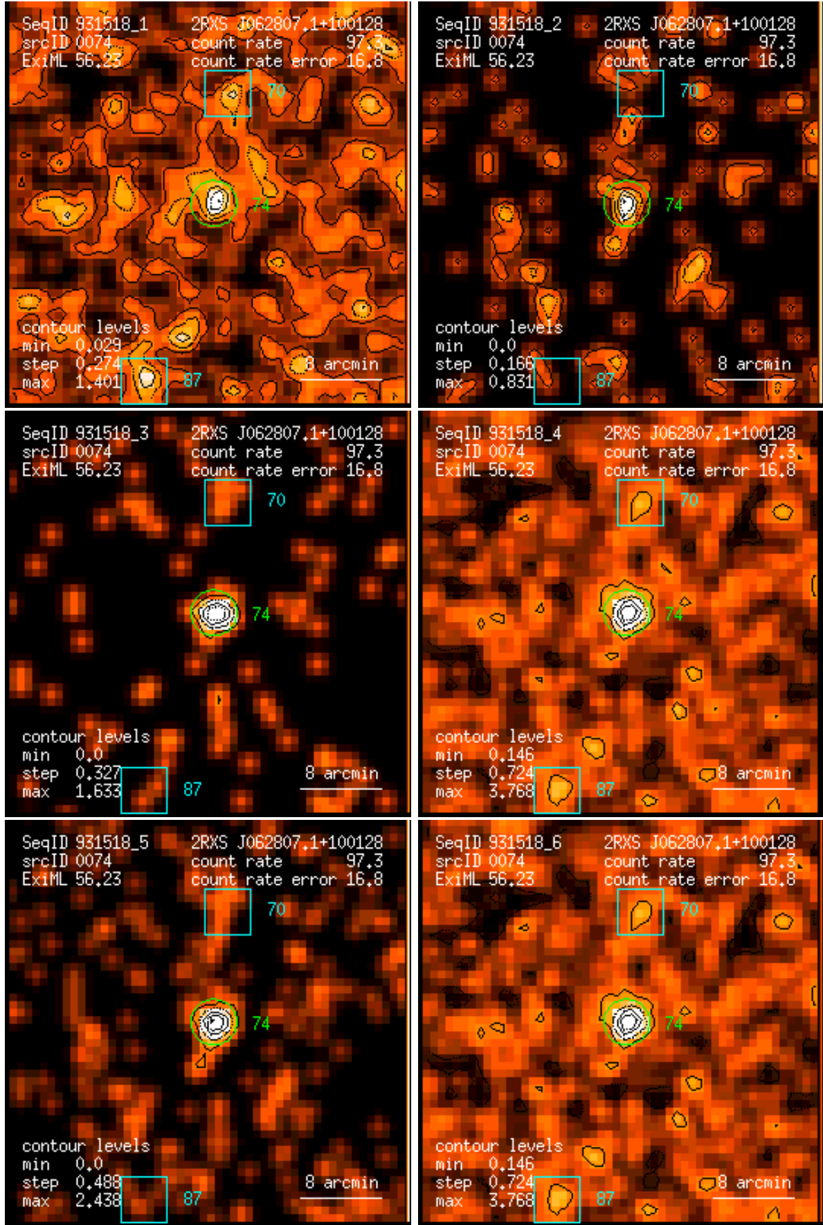
Figure 74: RASS 931518: detection 0074: band rate images, Gaussian filter: (1) PSPC channels 11 – 41, (2) 52 – 90, (3) 91 – 201, (4) 11 – 235, (5) 52 – 201, (6) 11 – 201. Broad band rates in counts/ks. Band rate contour levels in counts/ks/arcmin 2 .
