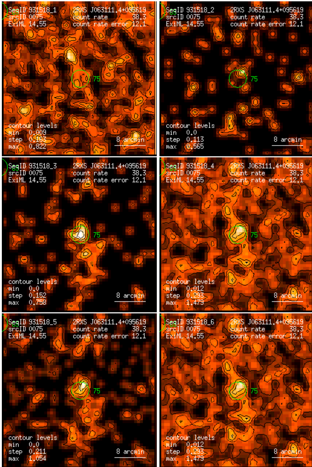
Figure 75: RASS 931518: detection 0075: band rate images, Gaussian filter: (1) PSPC channels 11 – 41, (2) 52 – 90, (3) 91 – 201, (4) 11 – 235, (5) 52 – 201, (6) 11 – 201. Broad band rates in counts/ks. Band rate contour levels in counts/ks/arcmin 2 .
