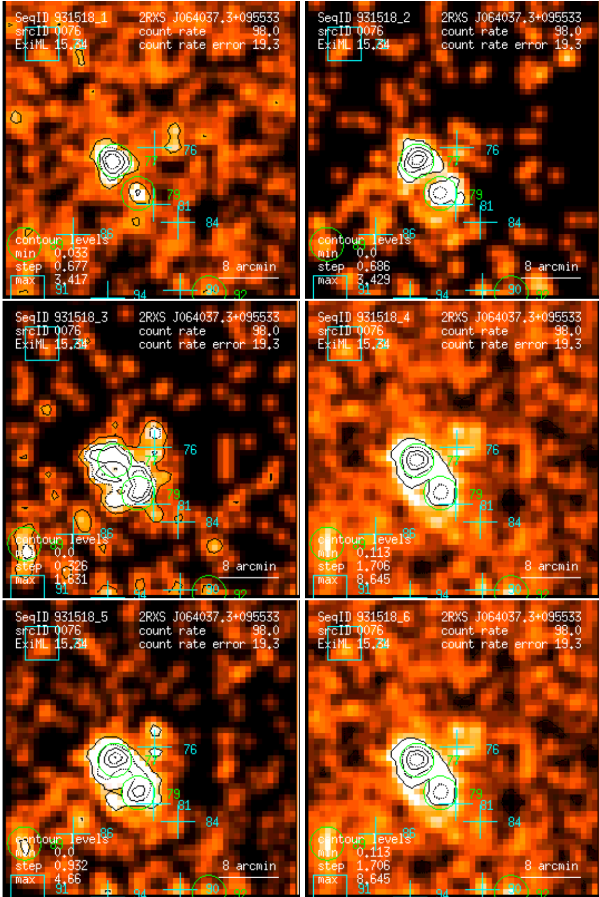
Figure 76: RASS 931518: detection 0076: band rate images, Gaussian filter: (1) PSPC channels 11 – 41, (2) 52 – 90, (3) 91 – 201, (4) 11 – 235, (5) 52 – 201, (6) 11 – 201. Broad band rates in counts/ks. Band rate contour levels in counts/ks/arcmin 2 .
