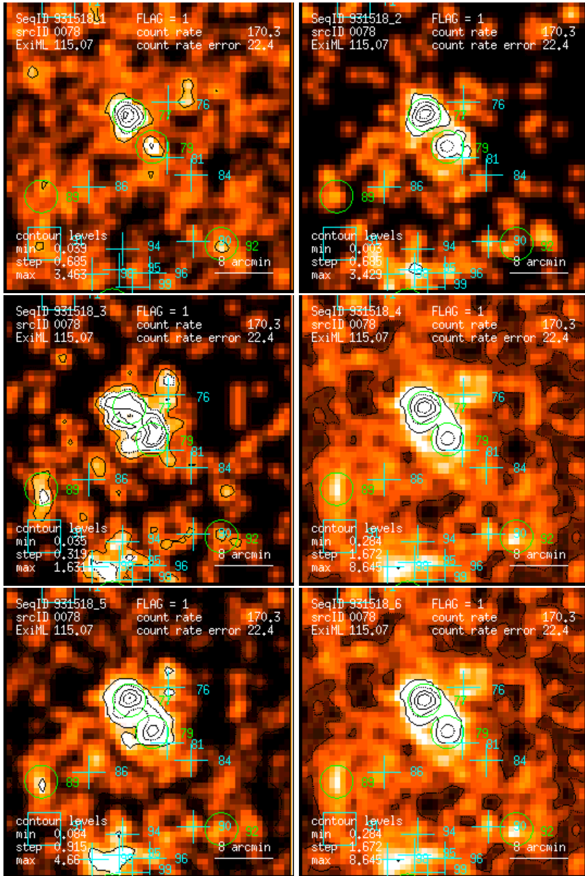
Figure 78: RASS 931518: detection 0078: band rate images, Gaussian filter: (1) PSPC channels 11 – 41, (2) 52 – 90, (3) 91 – 201, (4) 11 – 235, (5) 52 – 201, (6) 11 – 201. Broad band rates in counts/ks. Band rate contour levels in counts/ks/arcmin 2 .
