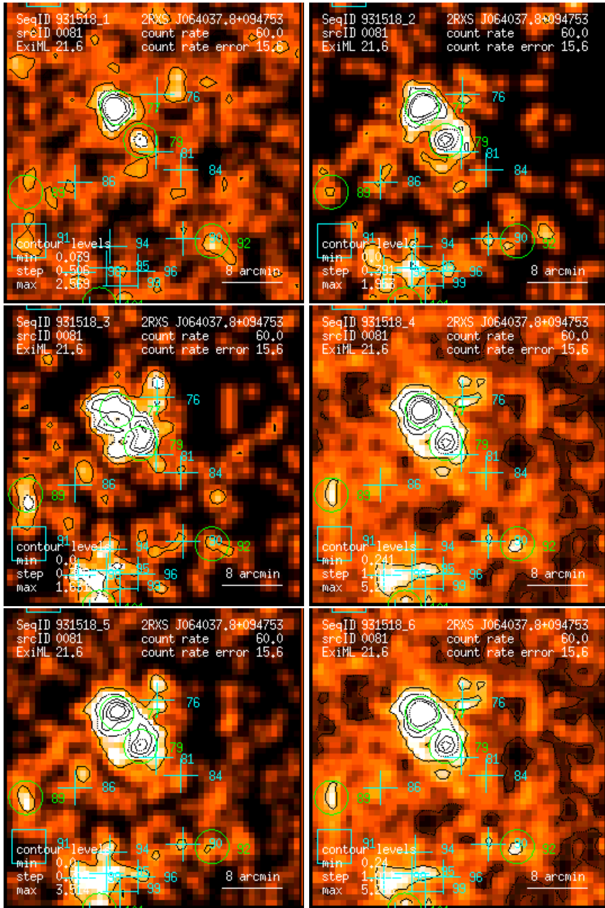
Figure 81: RASS 931518: detection 0081: band rate images, Gaussian filter: (1) PSPC channels 11 – 41, (2) 52 – 90, (3) 91 – 201, (4) 11 – 235, (5) 52 – 201, (6) 11 – 201. Broad band rates in counts/ks. Band rate contour levels in counts/ks/arcmin 2 .
