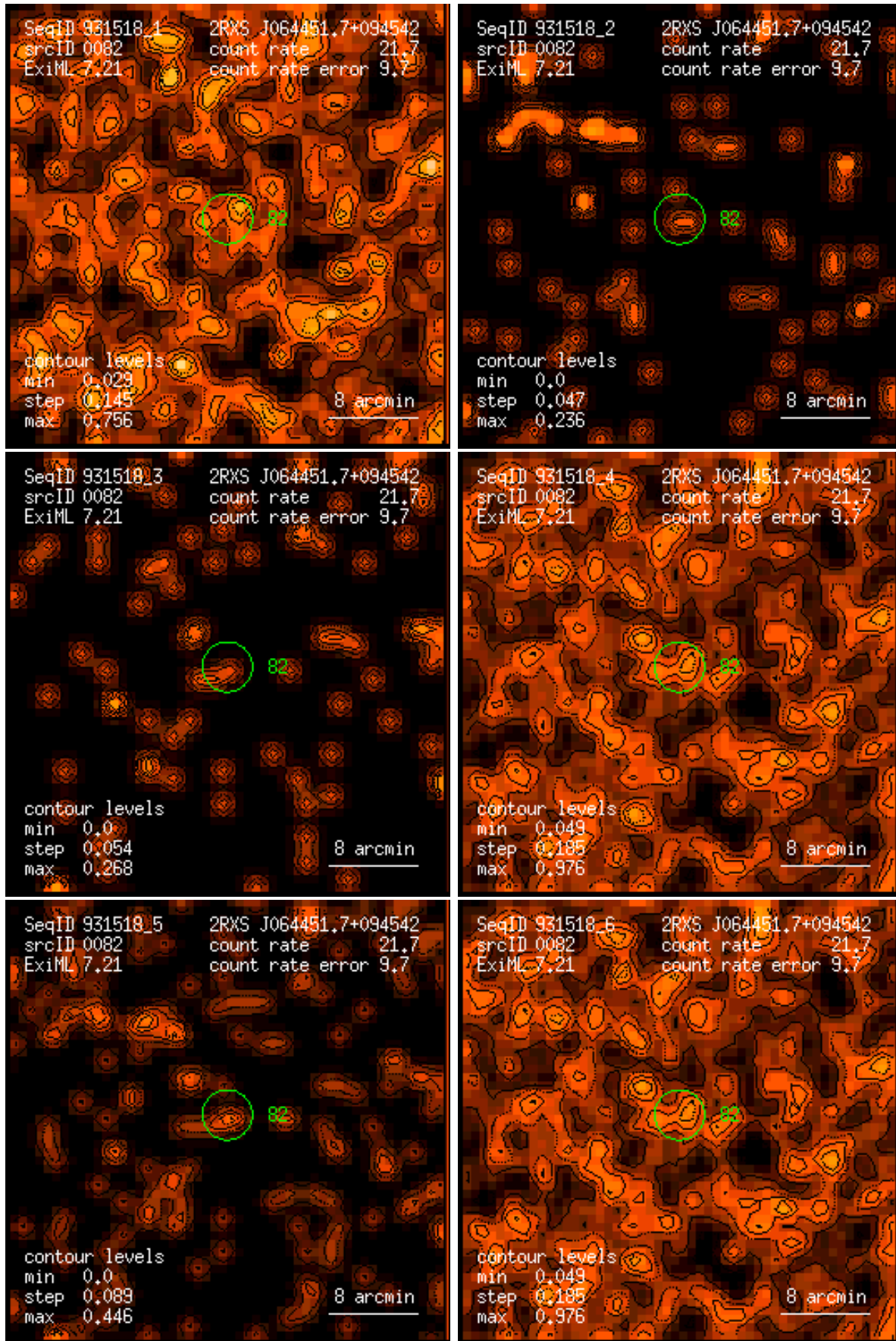
Figure 82: RASS 931518: detection 0082: band rate images, Gaussian filter: (1) PSPC channels 11 – 41, (2) 52 – 90, (3) 91 – 201, (4) 11 – 235, (5) 52 – 201, (6) 11 – 201. Broad band rates in counts/ks. Band rate contour levels in counts/ks/arcmin 2 .
