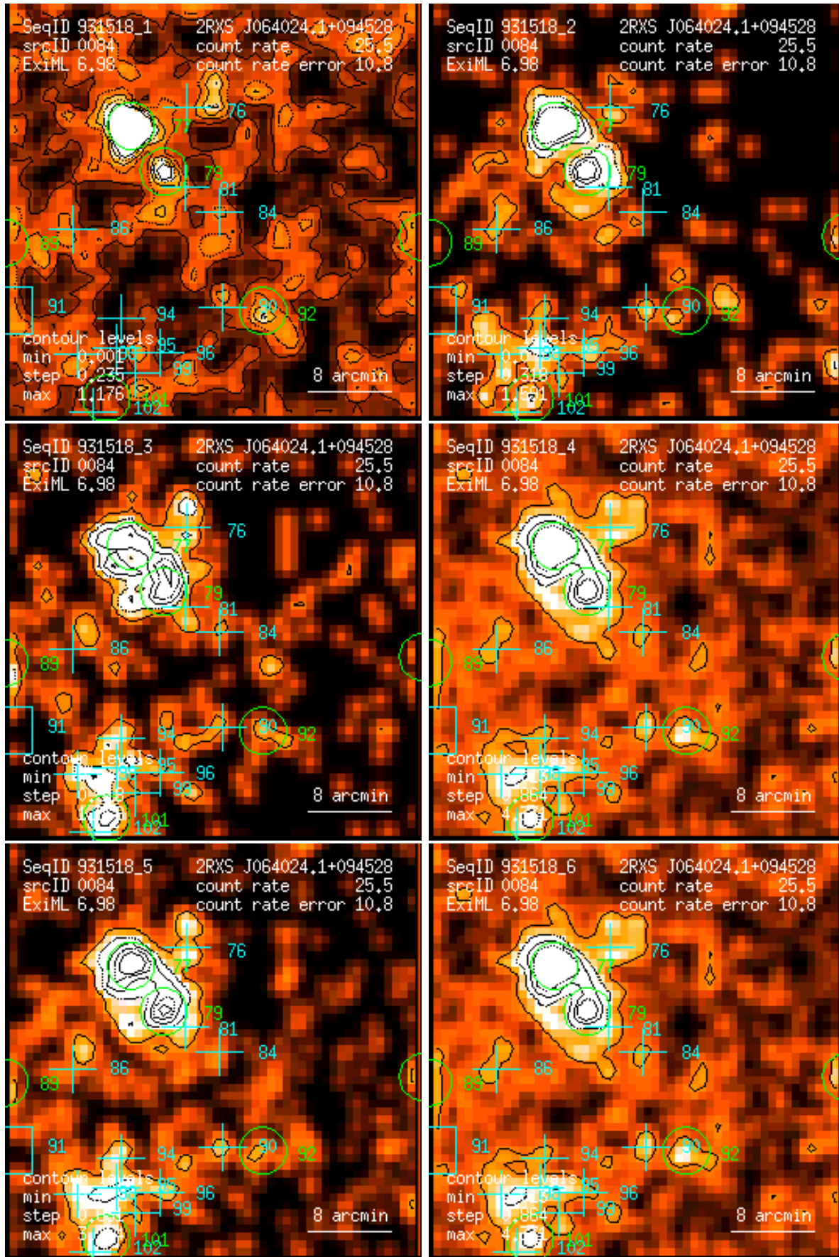
Figure 84: RASS 931518: detection 0084: band rate images, Gaussian filter: (1) PSPC channels 11 – 41, (2) 52 – 90, (3) 91 – 201, (4) 11 – 235, (5) 52 – 201, (6) 11 – 201. Broad band rates in counts/ks. Band rate contour levels in counts/ks/arcmin 2 .
