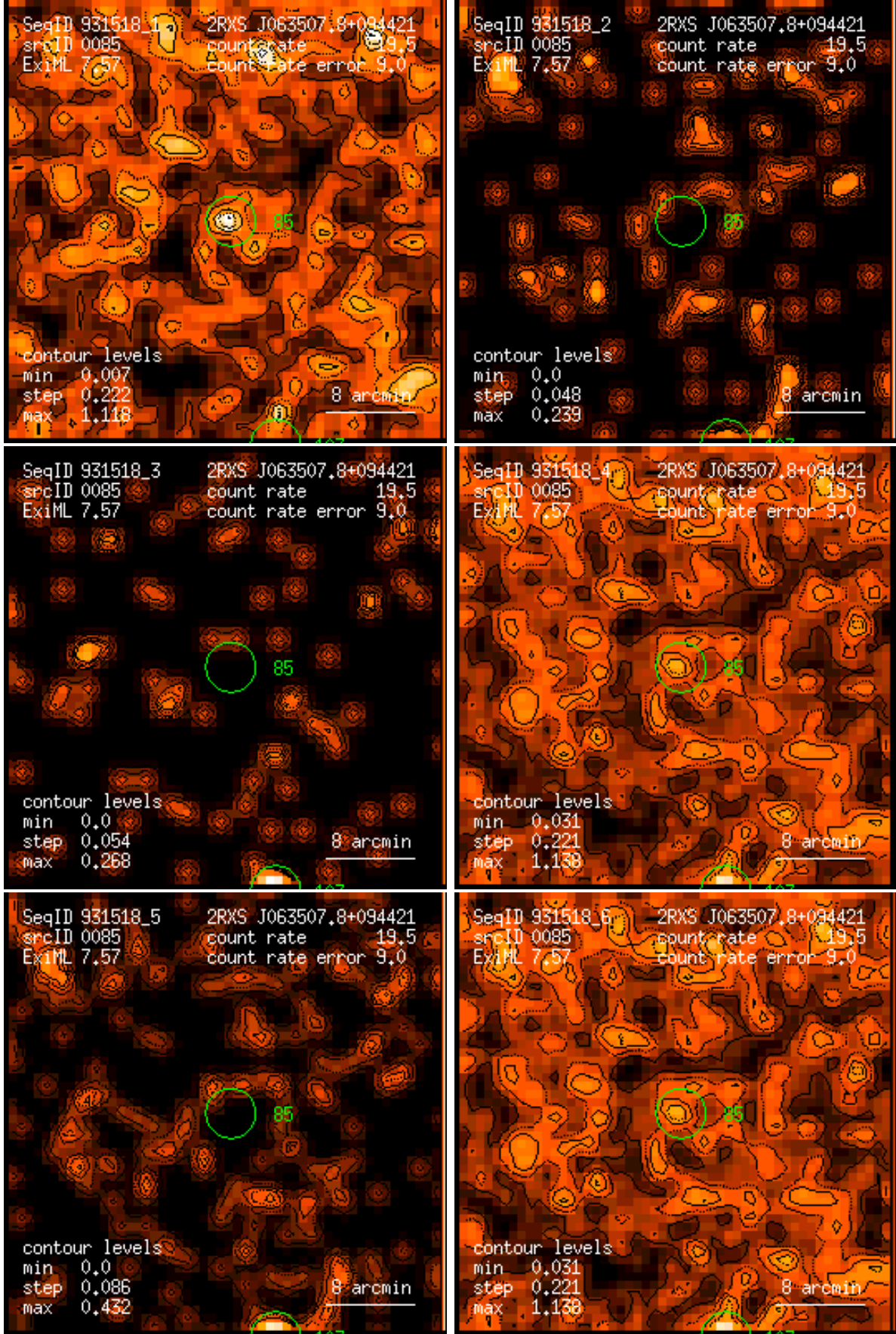
Figure 85: RASS 931518: detection 0085: band rate images, Gaussian filter: (1) PSPC channels 11 – 41, (2) 52 – 90, (3) 91 – 201, (4) 11 – 235, (5) 52 – 201, (6) 11 – 201. Broad band rates in counts/ks. Band rate contour levels in counts/ks/arcmin 2 .
