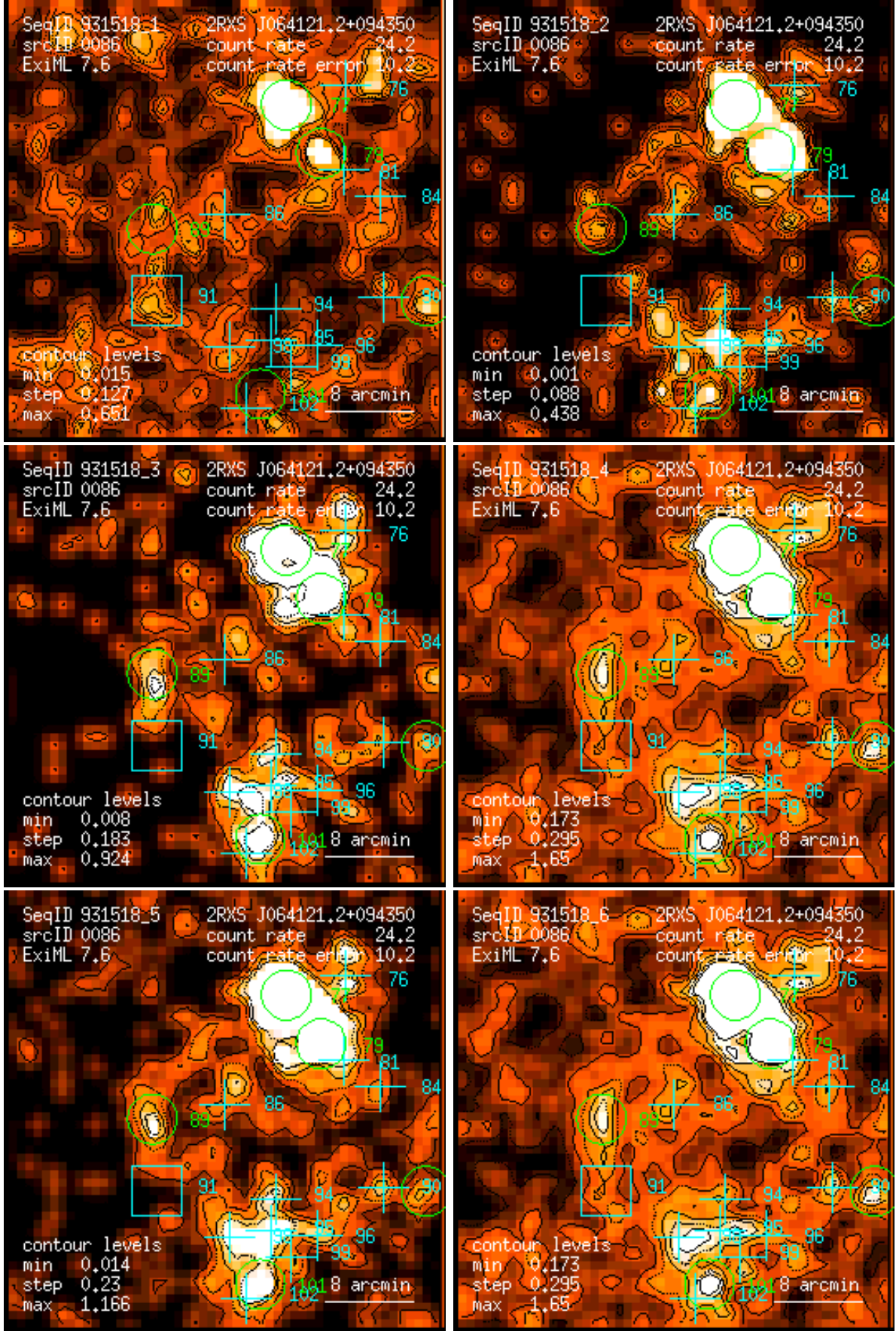
Figure 86: RASS 931518: detection 0086: band rate images, Gaussian filter: (1) PSPC channels 11 – 41, (2) 52 – 90, (3) 91 – 201, (4) 11 – 235, (5) 52 – 201, (6) 11 – 201. Broad band rates in counts/ks. Band rate contour levels in counts/ks/arcmin 2 .
