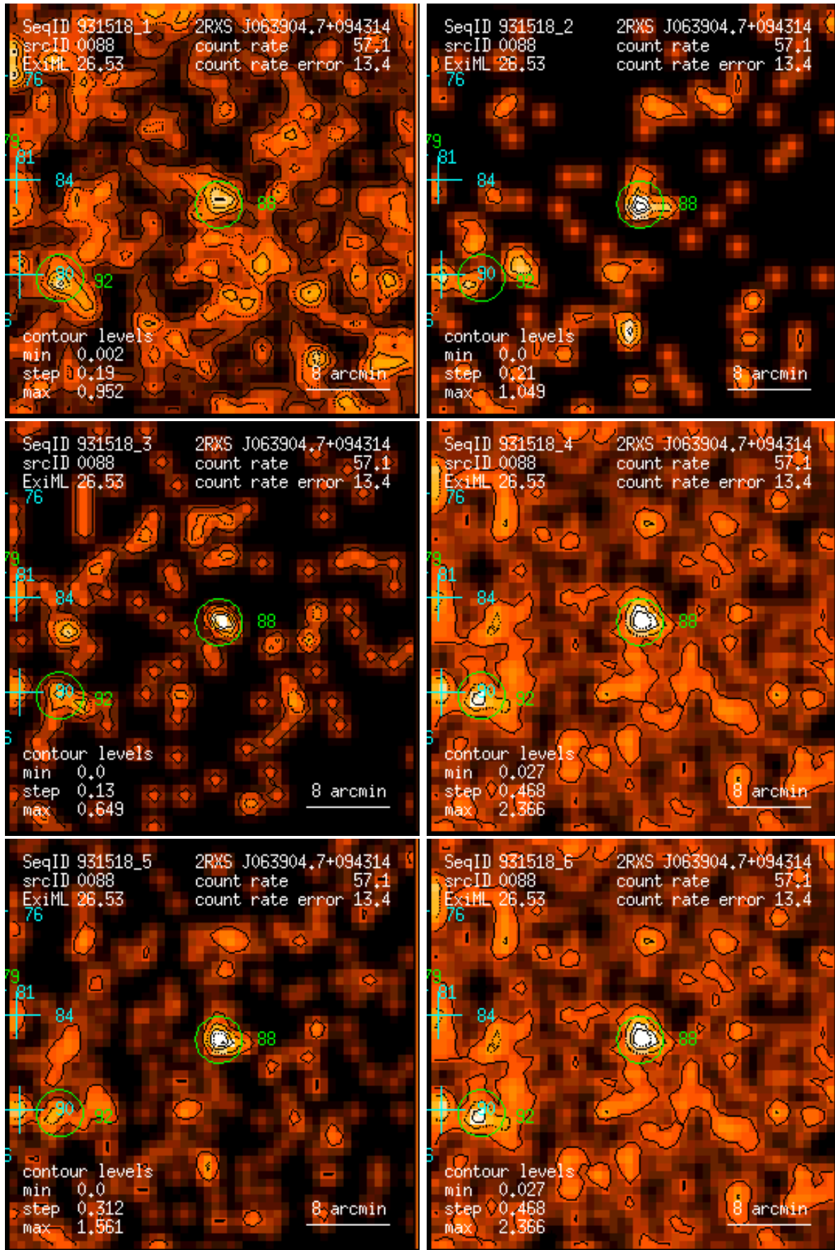
Figure 88: RASS 931518: detection 0088: band rate images, Gaussian filter: (1) PSPC channels 11 – 41, (2) 52 – 90, (3) 91 – 201, (4) 11 – 235, (5) 52 – 201, (6) 11 – 201. Broad band rates in counts/ks. Band rate contour levels in counts/ks/arcmin 2 .
