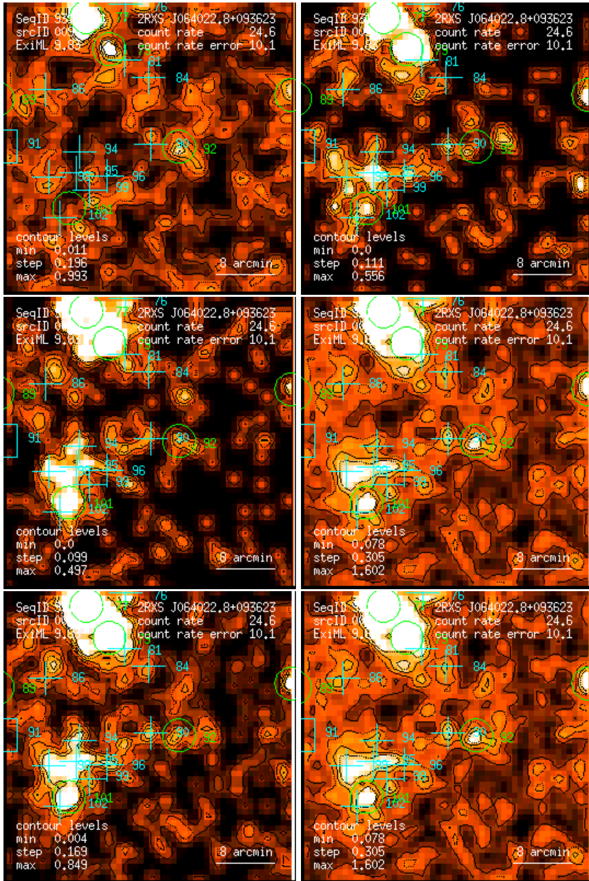
Figure 90: RASS 931518: detection 0090: band rate images, Gaussian filter: (1) PSPC channels 11 – 41, (2) 52 – 90, (3) 91 – 201, (4) 11 – 235, (5) 52 – 201, (6) 11 – 201. Broad band rates in counts/ks. Band rate contour levels in counts/ks/arcmin 2 .
