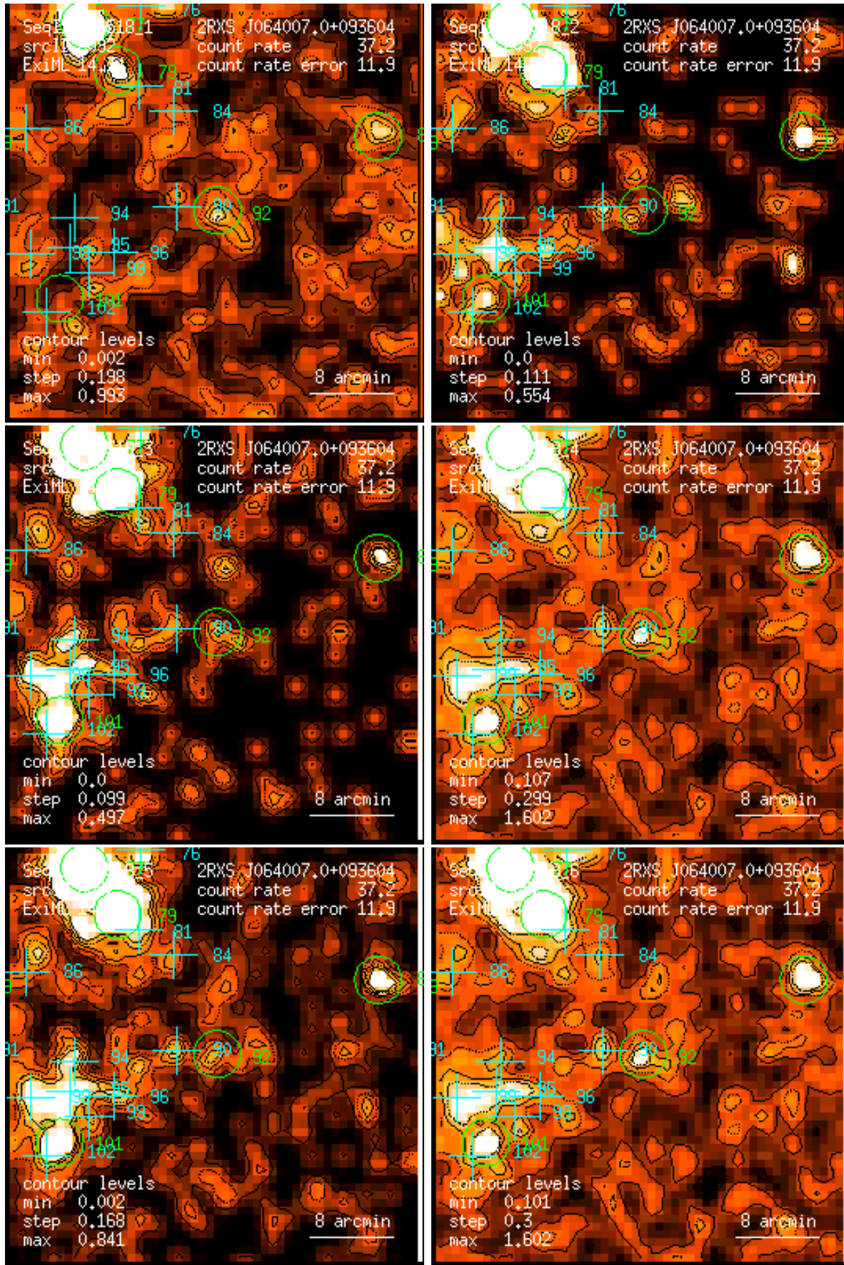
Figure 92: RASS 931518: detection 0092: band rate images, Gaussian filter: (1) PSPC channels 11 – 41, (2) 52 – 90, (3) 91 – 201, (4) 11 – 235, (5) 52 – 201, (6) 11 – 201. Broad band rates in counts/ks. Band rate contour levels in counts/ks/arcmin 2 .
