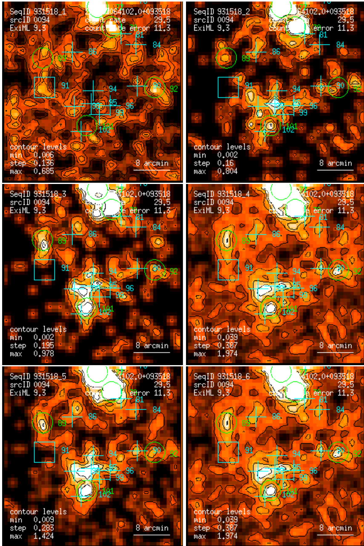
Figure 94: RASS 931518: detection 0094: band rate images, Gaussian filter: (1) PSPC channels 11 – 41, (2) 52 – 90, (3) 91 – 201, (4) 11 – 235, (5) 52 – 201, (6) 11 – 201. Broad band rates in counts/ks. Band rate contour levels in counts/ks/arcmin 2 .
