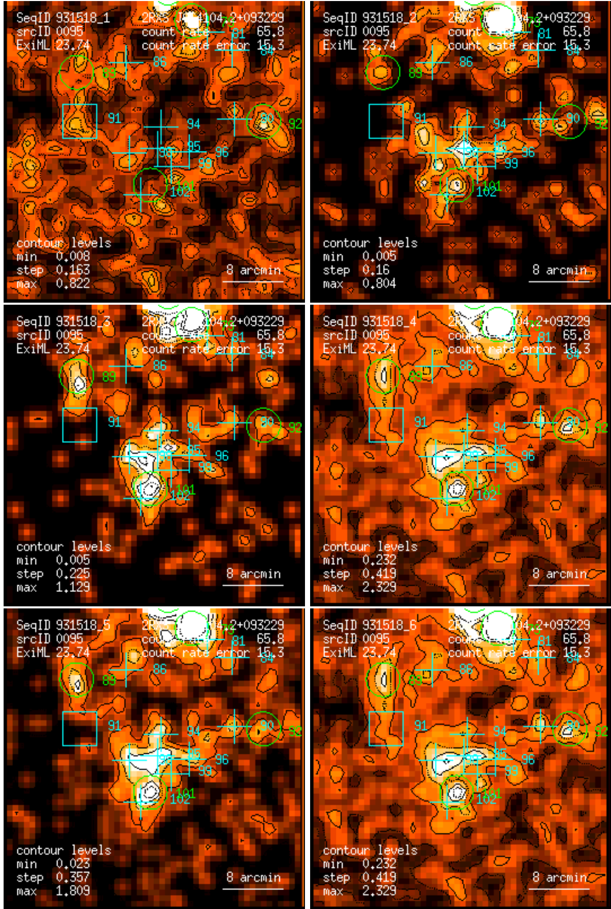
Figure 95: RASS 931518: detection 0095: band rate images, Gaussian filter: (1) PSPC channels 11 – 41, (2) 52 – 90, (3) 91 – 201, (4) 11 – 235, (5) 52 – 201, (6) 11 – 201. Broad band rates in counts/ks. Band rate contour levels in counts/ks/arcmin 2 .
