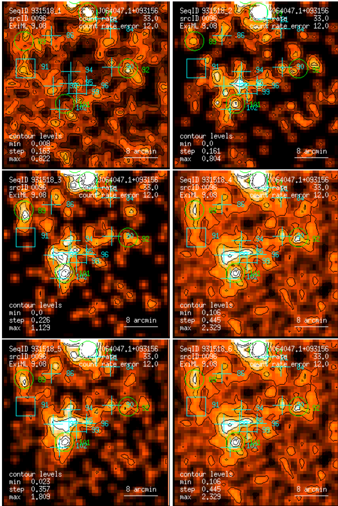
Figure 96: RASS 931518: detection 0096: band rate images, Gaussian filter: (1) PSPC channels 11 – 41, (2) 52 – 90, (3) 91 – 201, (4) 11 – 235, (5) 52 – 201, (6) 11 – 201. Broad band rates in counts/ks. Band rate contour levels in counts/ks/arcmin 2 .
