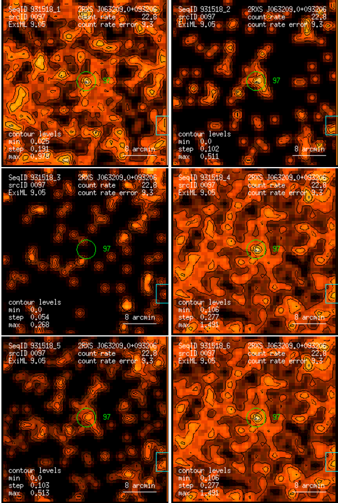
Figure 97: RASS 931518: detection 0097: band rate images, Gaussian filter: (1) PSPC channels 11 – 41, (2) 52 – 90, (3) 91 – 201, (4) 11 – 235, (5) 52 – 201, (6) 11 – 201. Broad band rates in counts/ks. Band rate contour levels in counts/ks/arcmin 2 .
