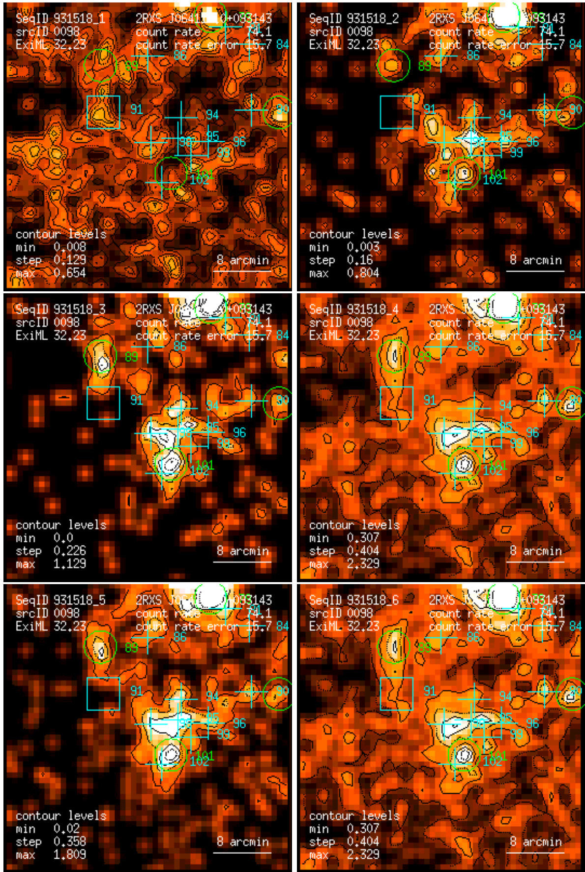
Figure 98: RASS 931518: detection 0098: band rate images, Gaussian filter: (1) PSPC channels 11 – 41, (2) 52 – 90, (3) 91 – 201, (4) 11 – 235, (5) 52 – 201, (6) 11 – 201. Broad band rates in counts/ks. Band rate contour levels in counts/ks/arcmin 2 .
