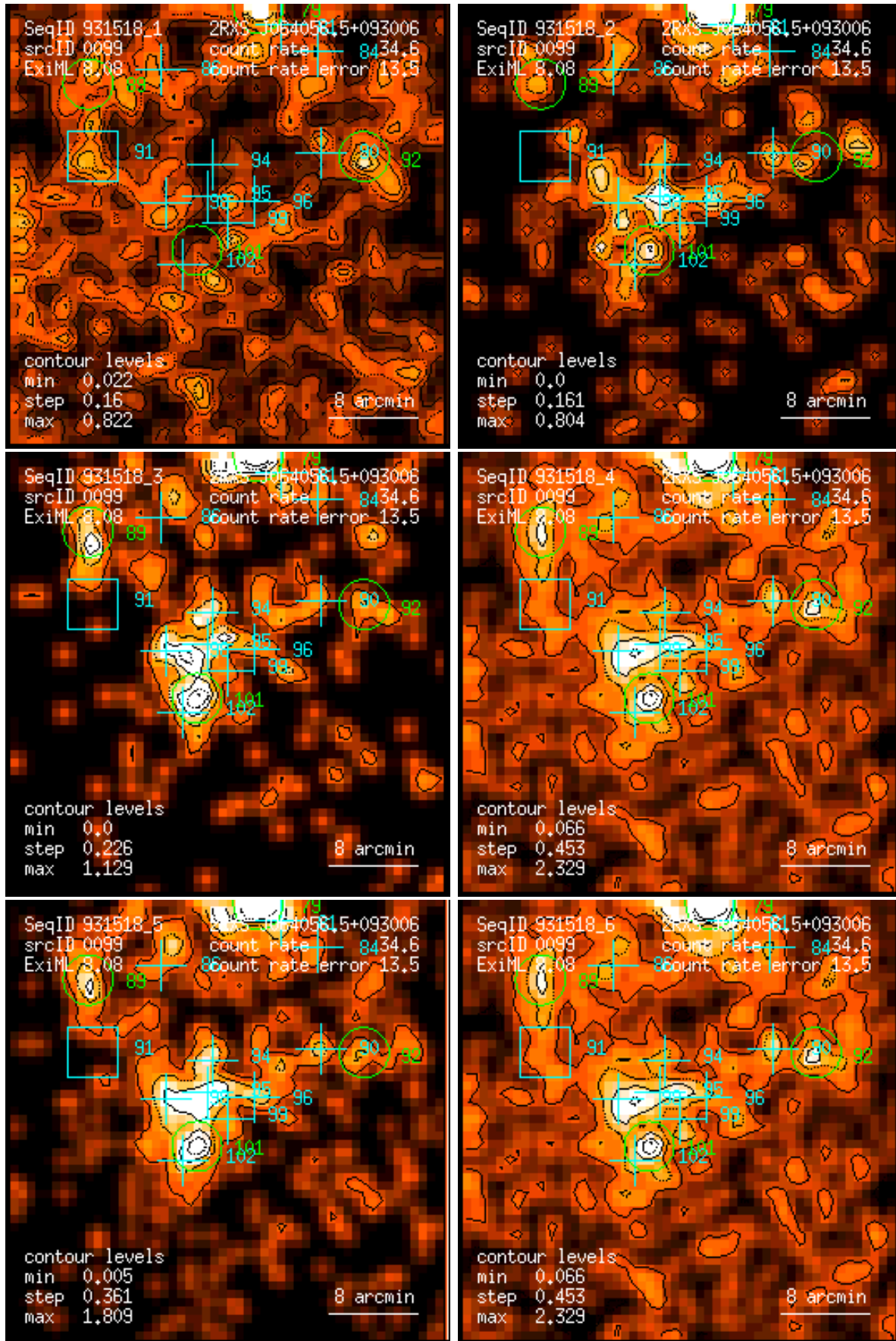
Figure 99: RASS 931518: detection 0099: band rate images, Gaussian filter: (1) PSPC channels 11 – 41, (2) 52 – 90, (3) 91 – 201, (4) 11 – 235, (5) 52 – 201, (6) 11 – 201. Broad band rates in counts/ks. Band rate contour levels in counts/ks/arcmin 2 .
