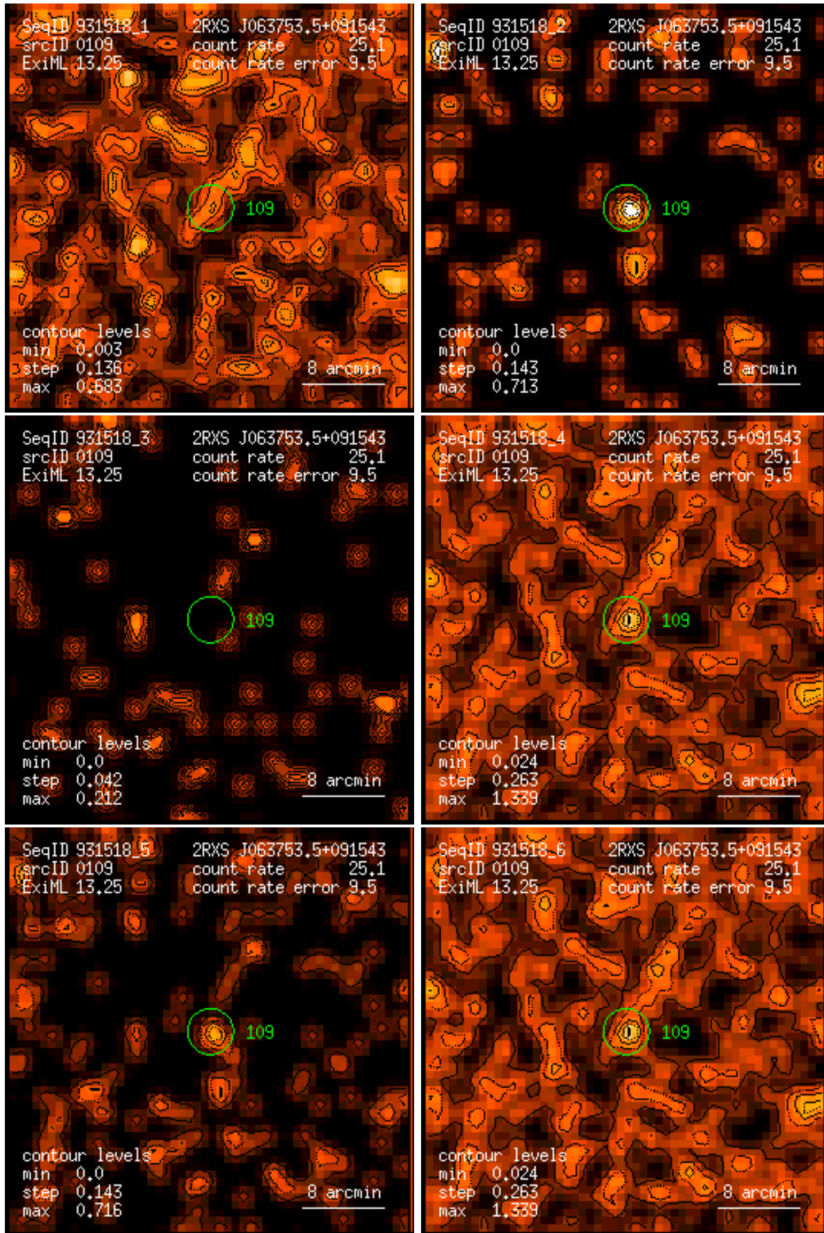
Figure 109: RASS 931518: detection 0109: band rate images, Gaussian filter: (1) PSPC channels 11 – 41, (2) 52 – 90, (3) 91 – 201, (4) 11 – 235, (5) 52 – 201, (6) 11 – 201. Broad band rates in counts/ks. Band rate contour levels in counts/ks/arcmin 2 .
