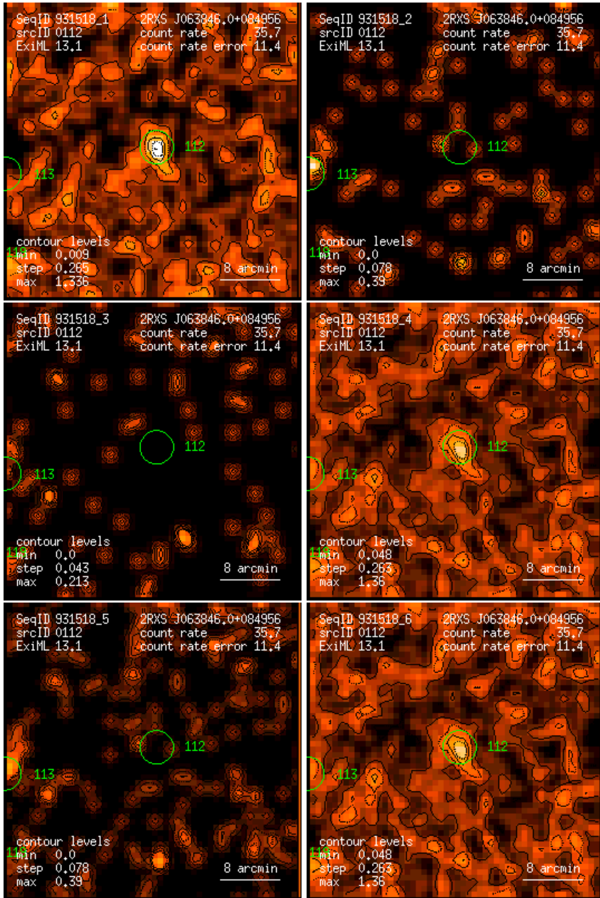
Figure 112: RASS 931518: detection 0112: band rate images, Gaussian filter: (1) PSPC channels 11 – 41, (2) 52 – 90, (3) 91 – 201, (4) 11 – 235, (5) 52 – 201, (6) 11 – 201. Broad band rates in counts/ks. Band rate contour levels in counts/ks/arcmin 2 .
