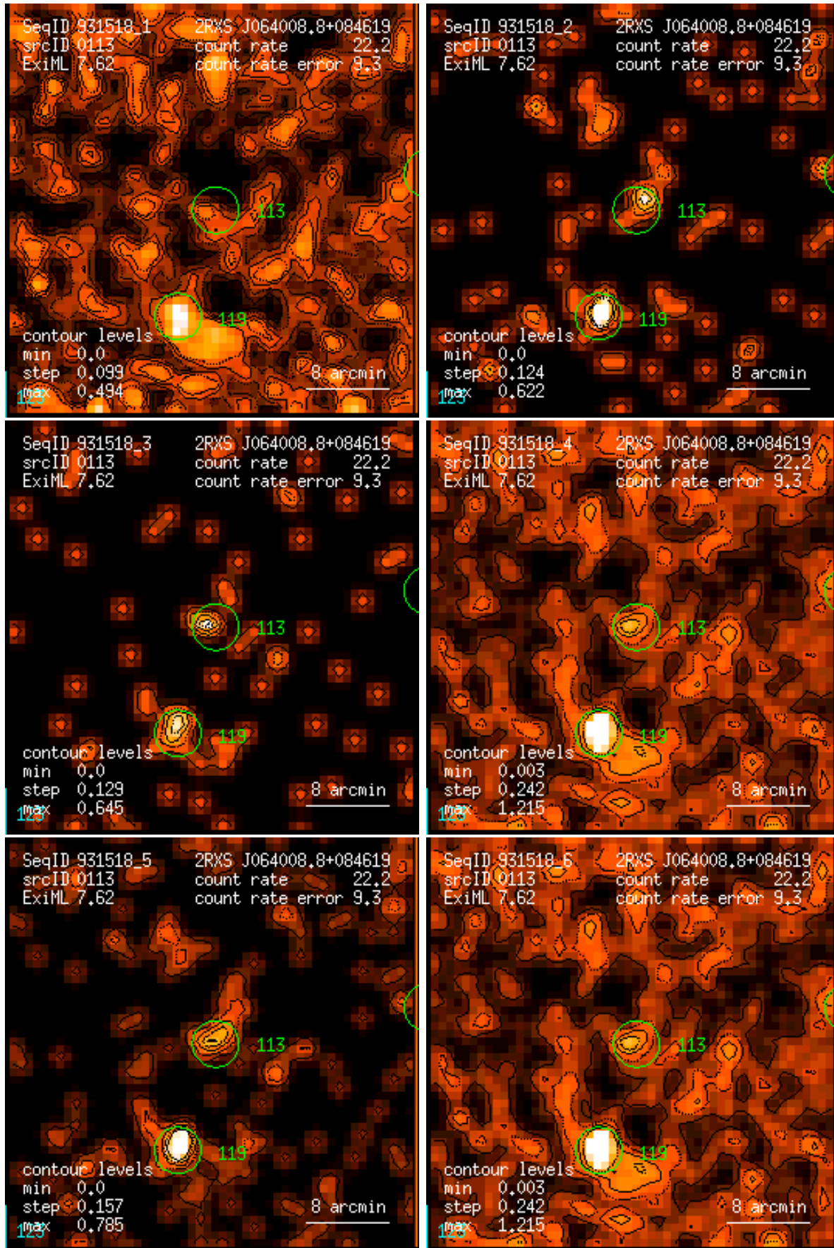
Figure 113: RASS 931518: detection 0113: band rate images, Gaussian filter: (1) PSPC channels 11 – 41, (2) 52 – 90, (3) 91 – 201, (4) 11 – 235, (5) 52 – 201, (6) 11 – 201. Broad band rates in counts/ks. Band rate contour levels in counts/ks/arcmin 2 .
