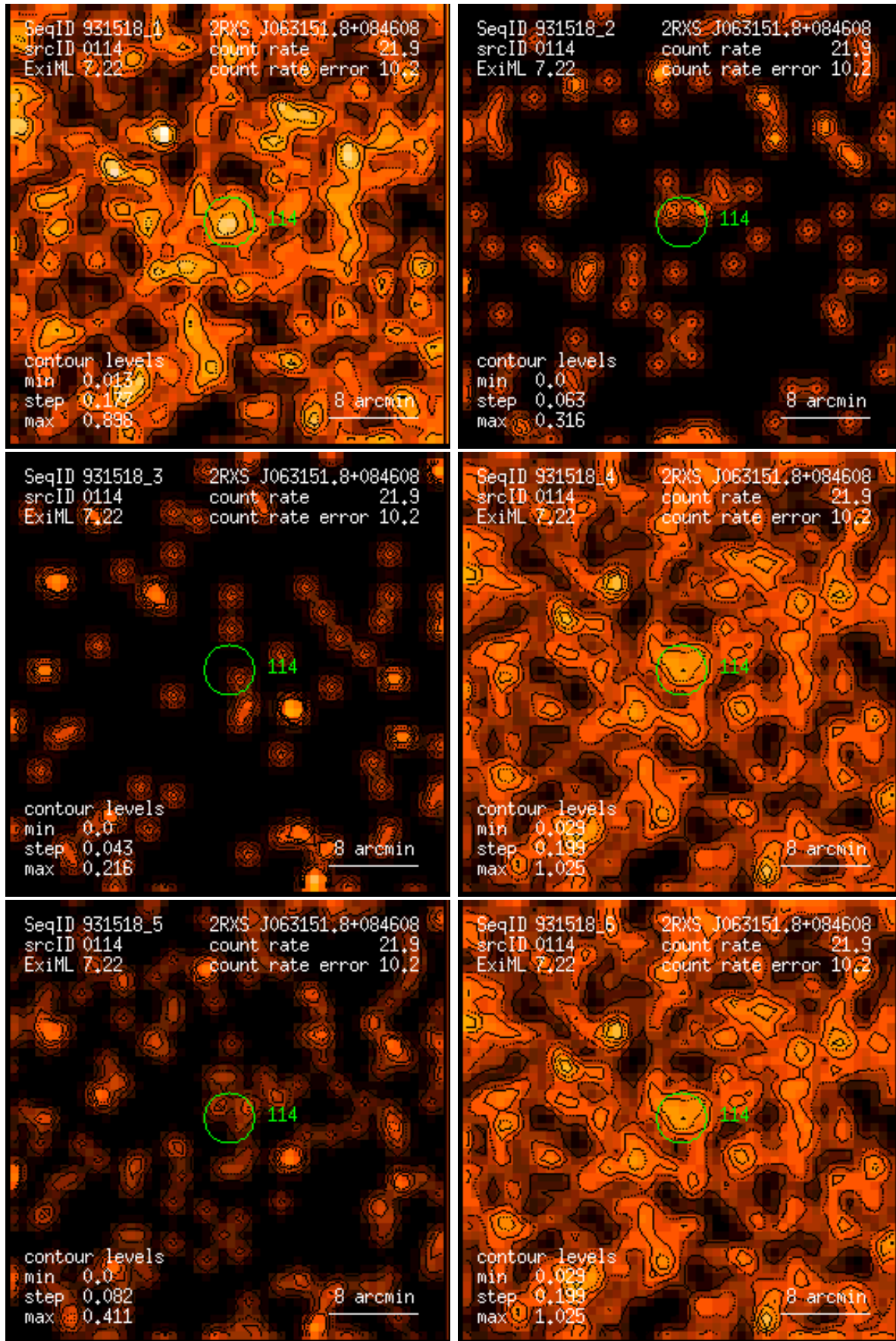
Figure 114: RASS 931518: detection 0114: band rate images, Gaussian filter: (1) PSPC channels 11 – 41, (2) 52 – 90, (3) 91 – 201, (4) 11 – 235, (5) 52 – 201, (6) 11 – 201. Broad band rates in counts/ks. Band rate contour levels in counts/ks/arcmin 2 .
