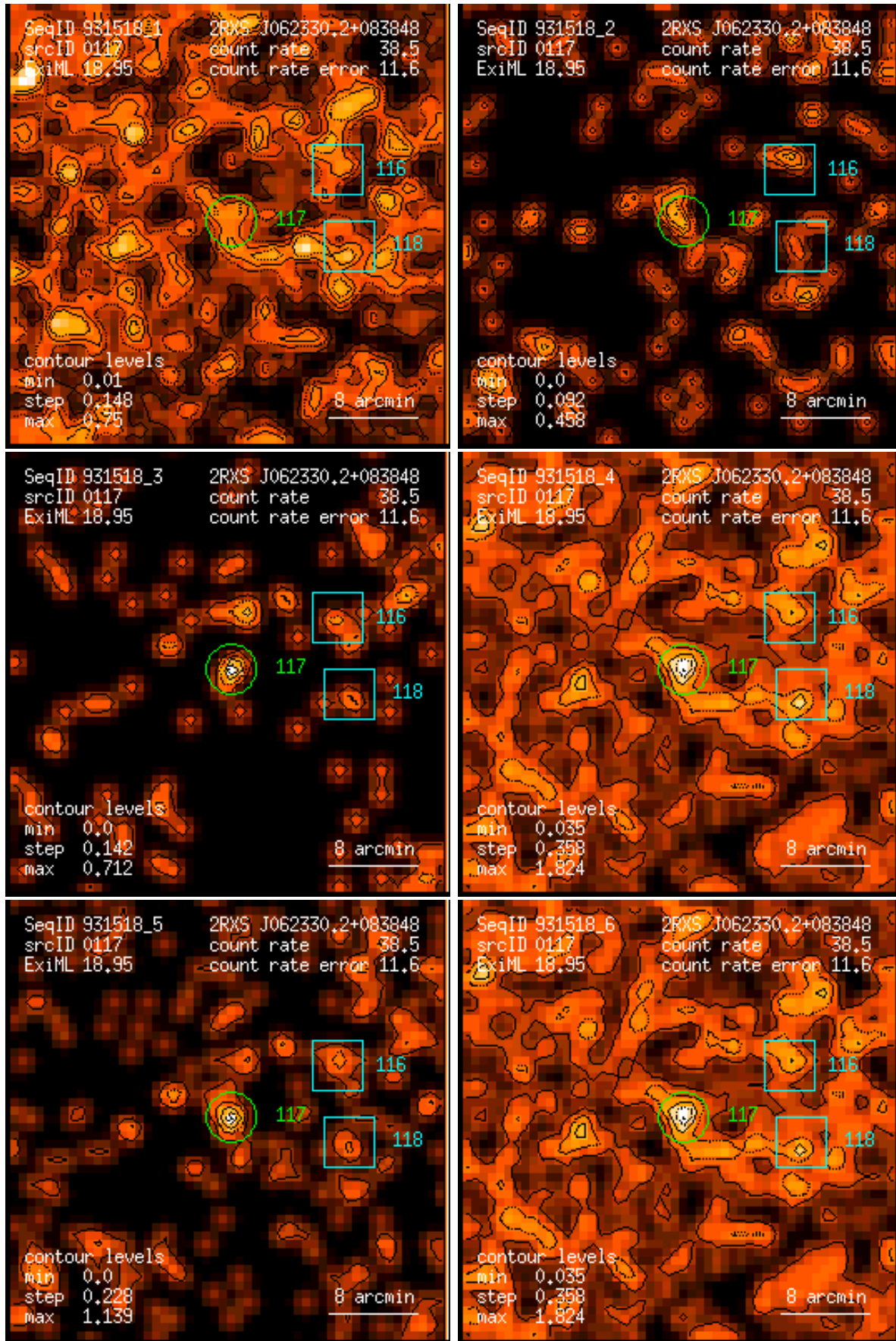
Figure 117: RASS 931518: detection 0117: band rate images, Gaussian filter: (1) PSPC channels 11 – 41, (2) 52 – 90, (3) 91 – 201, (4) 11 – 235, (5) 52 – 201, (6) 11 – 201. Broad band rates in counts/ks. Band rate contour levels in counts/ks/arcmin 2 .
