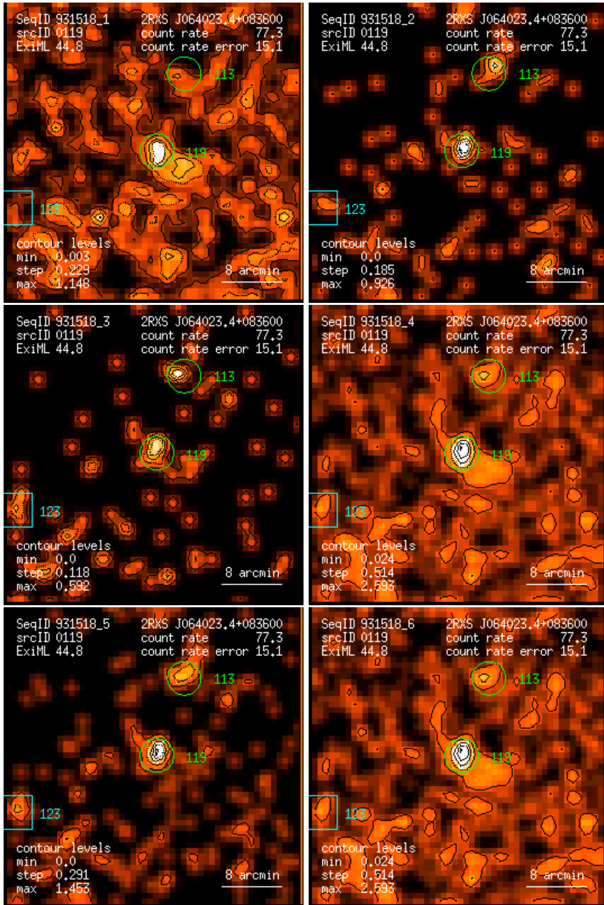
Figure 119: RASS 931518: detection 0119: band rate images, Gaussian filter: (1) PSPC channels 11 – 41, (2) 52 – 90, (3) 91 – 201, (4) 11 – 235, (5) 52 – 201, (6) 11 – 201. Broad band rates in counts/ks. Band rate contour levels in counts/ks/arcmin 2 .
