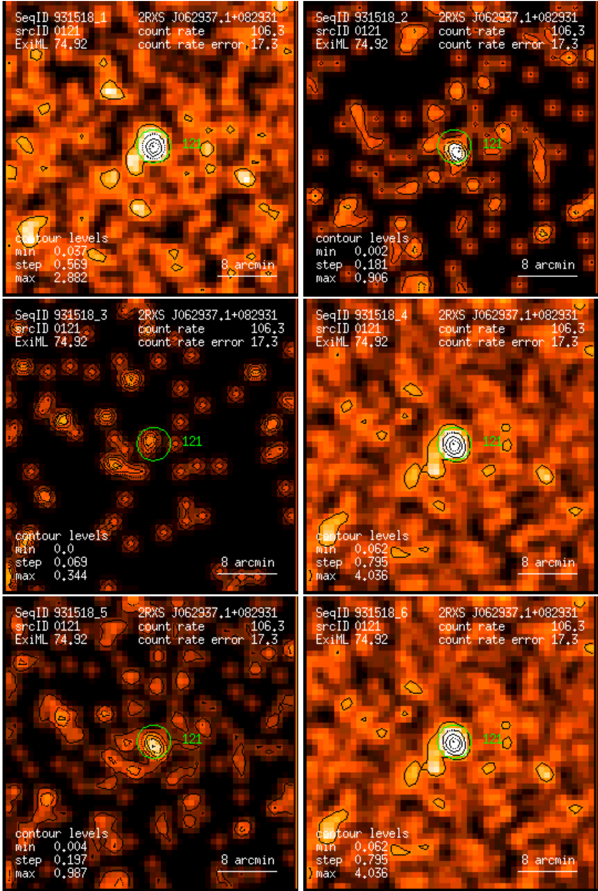
Figure 121: RASS 931518: detection 0121: band rate images, Gaussian filter: (1) PSPC channels 11 – 41, (2) 52 – 90, (3) 91 – 201, (4) 11 – 235, (5) 52 – 201, (6) 11 – 201. Broad band rates in counts/ks. Band rate contour levels in counts/ks/arcmin 2 .
