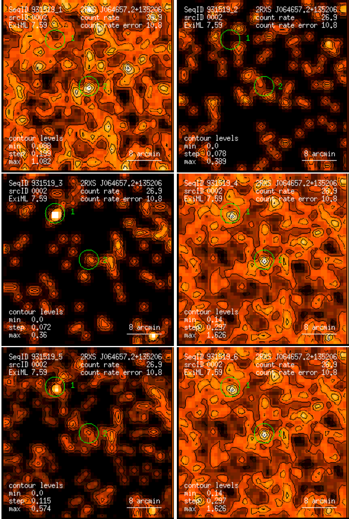
Figure 2: RASS 931519: detection 0002: band rate images, Gaussian filter: (1) PSPC channels 11 – 41, (2) 52 – 90, (3) 91 – 201, (4) 11 – 235, (5) 52 – 201, (6) 11 – 201. Broad band rates in counts/ks. Band rate contour levels in counts/ks/arcmin 2 .
