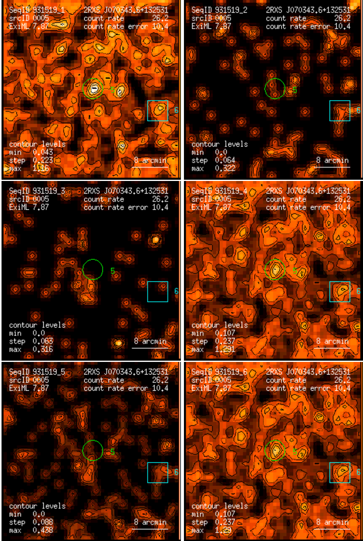
Figure 5: RASS 931519: detection 0005: band rate images, Gaussian filter: (1) PSPC channels 11 – 41, (2) 52 – 90, (3) 91 – 201, (4) 11 – 235, (5) 52 – 201, (6) 11 – 201. Broad band rates in counts/ks. Band rate contour levels in counts/ks/arcmin 2 .
