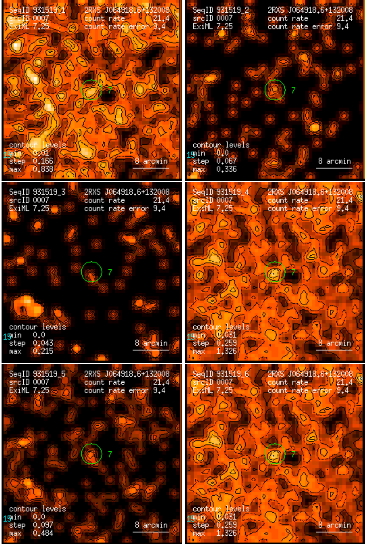
Figure 7: RASS 931519: detection 0007: band rate images, Gaussian filter: (1) PSPC channels 11 – 41, (2) 52 – 90, (3) 91 – 201, (4) 11 – 235, (5) 52 – 201, (6) 11 – 201. Broad band rates in counts/ks. Band rate contour levels in counts/ks/arcmin 2 .
