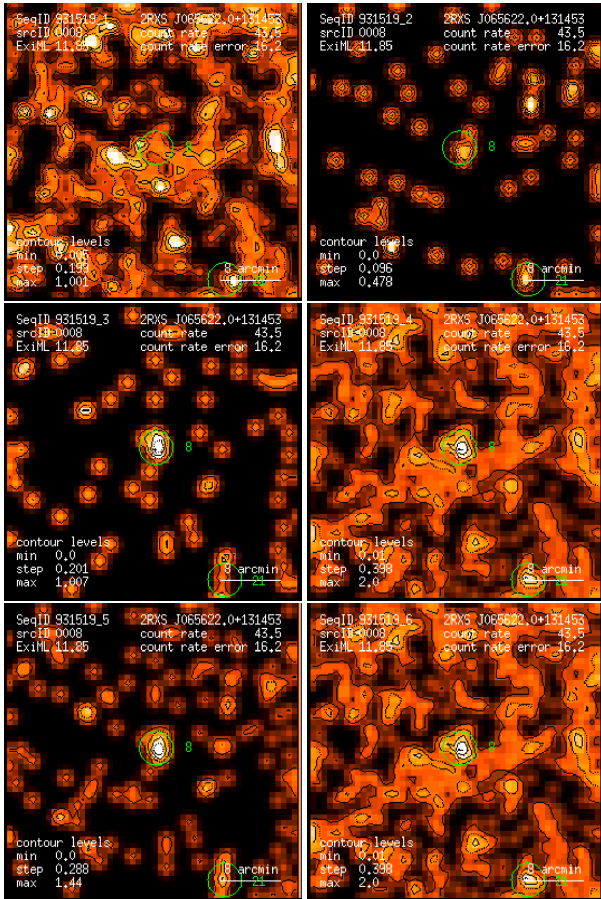
Figure 8: RASS 931519: detection 0008: band rate images, Gaussian filter: (1) PSPC channels 11 – 41, (2) 52 – 90, (3) 91 – 201, (4) 11 – 235, (5) 52 – 201, (6) 11 – 201. Broad band rates in counts/ks. Band rate contour levels in counts/ks/arcmin 2 .
