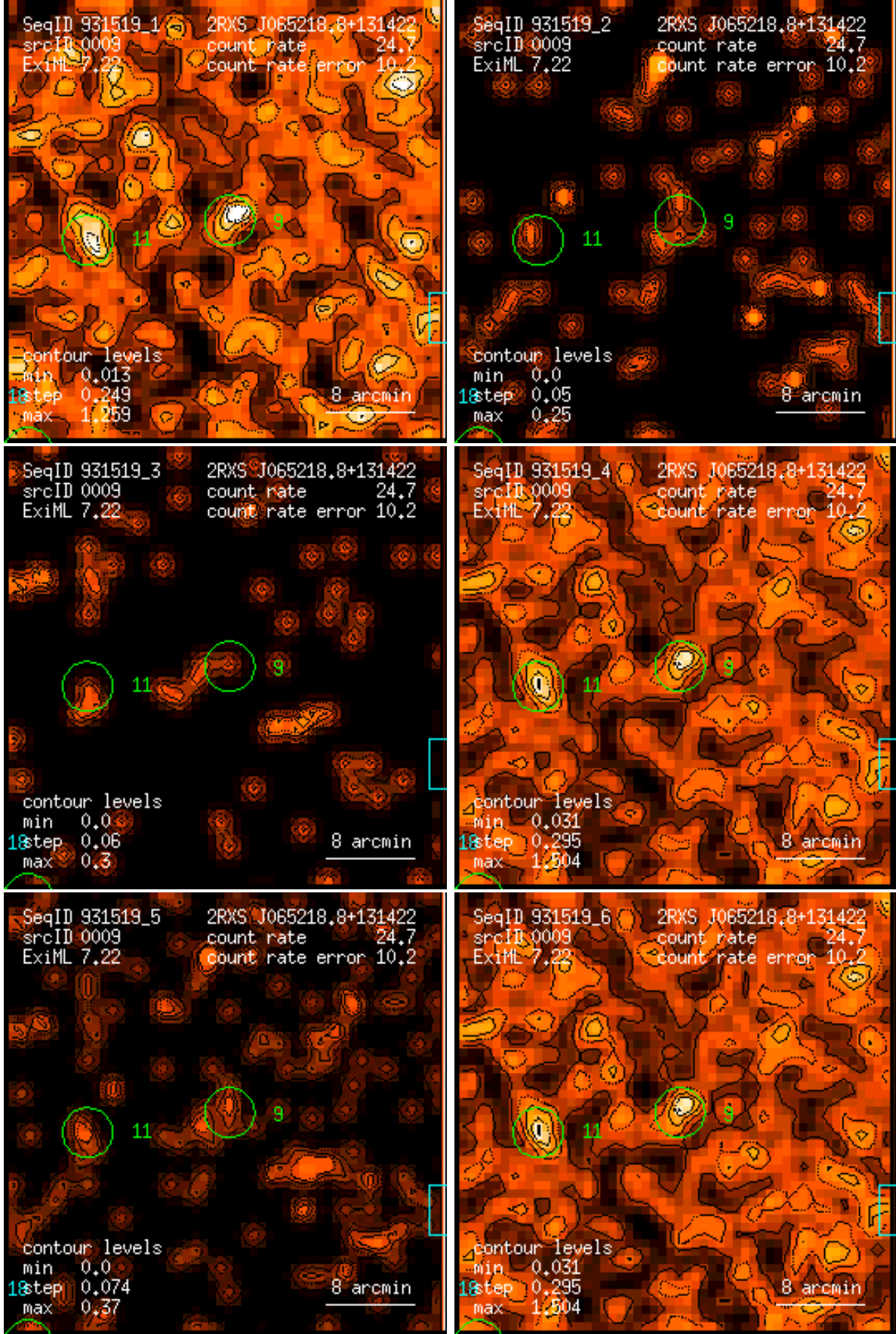
Figure 9: RASS 931519: detection 0009: band rate images, Gaussian filter: (1) PSPC channels 11 – 41, (2) 52 – 90, (3) 91 – 201, (4) 11 – 235, (5) 52 – 201, (6) 11 – 201. Broad band rates in counts/ks. Band rate contour levels in counts/ks/arcmin 2 .
