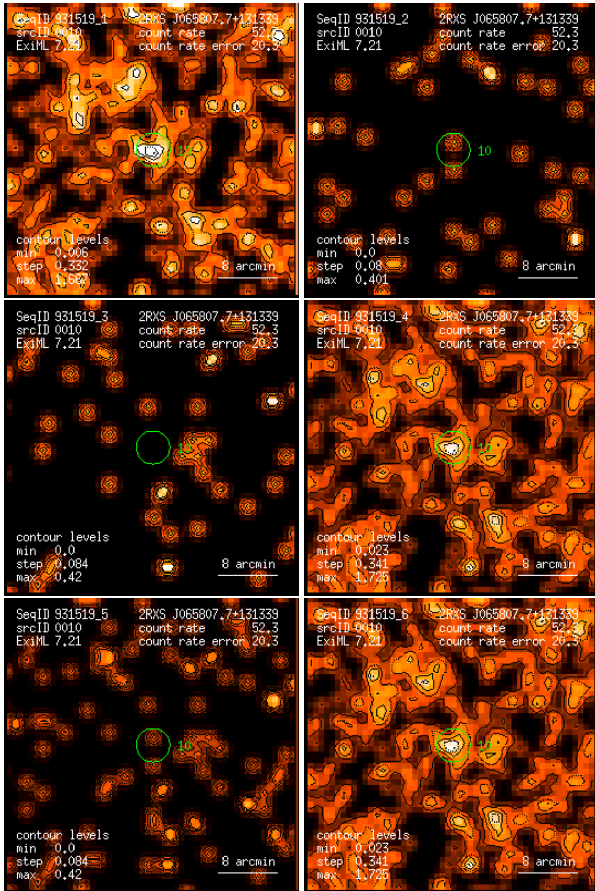
Figure 10: RASS 931519: detection 0010: band rate images, Gaussian filter: (1) PSPC channels 11 – 41, (2) 52 – 90, (3) 91 – 201, (4) 11 – 235, (5) 52 – 201, (6) 11 – 201. Broad band rates in counts/ks. Band rate contour levels in counts/ks/arcmin 2 .
