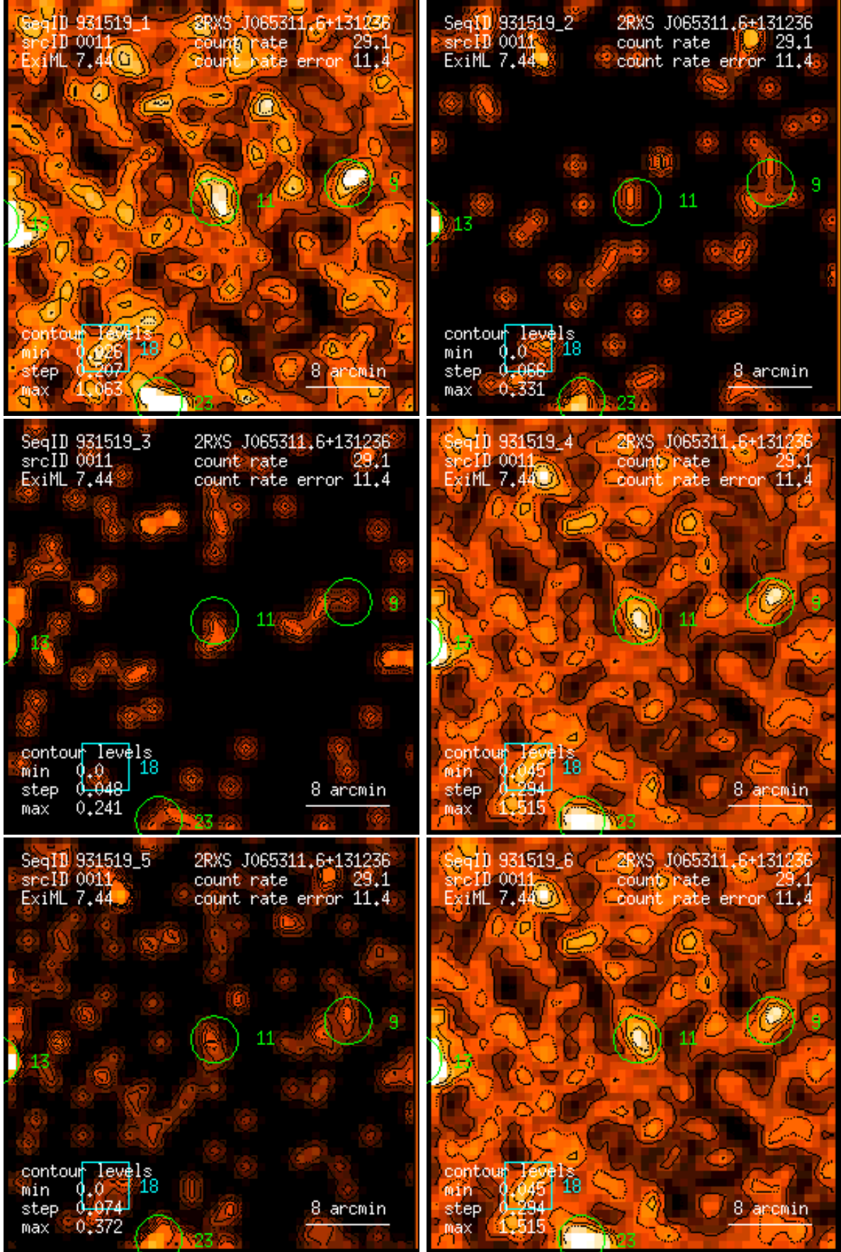
Figure 11: RASS 931519: detection 0011: band rate images, Gaussian filter: (1) PSPC channels 11 – 41, (2) 52 – 90, (3) 91 – 201, (4) 11 – 235, (5) 52 – 201, (6) 11 – 201. Broad band rates in counts/ks. Band rate contour levels in counts/ks/arcmin 2 .
