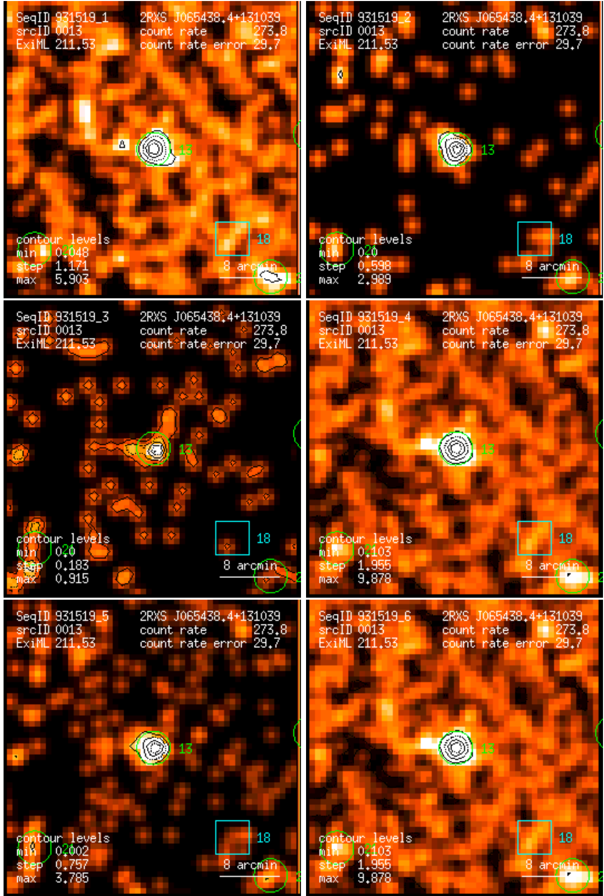
Figure 13: RASS 931519: detection 0013: band rate images, Gaussian filter: (1) PSPC channels 11 – 41, (2) 52 – 90, (3) 91 – 201, (4) 11 – 235, (5) 52 – 201, (6) 11 – 201. Broad band rates in counts/ks. Band rate contour levels in counts/ks/arcmin 2 .
