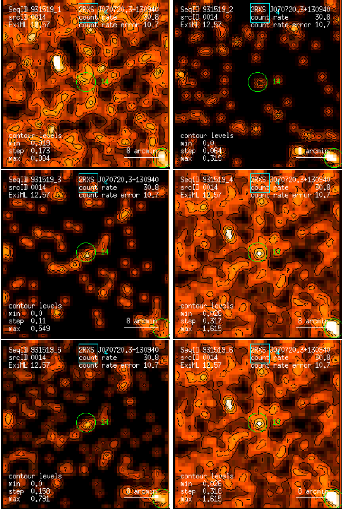
Figure 14: RASS 931519: detection 0014: band rate images, Gaussian filter: (1) PSPC channels 11 – 41, (2) 52 – 90, (3) 91 – 201, (4) 11 – 235, (5) 52 – 201, (6) 11 – 201. Broad band rates in counts/ks. Band rate contour levels in counts/ks/arcmin 2 .
