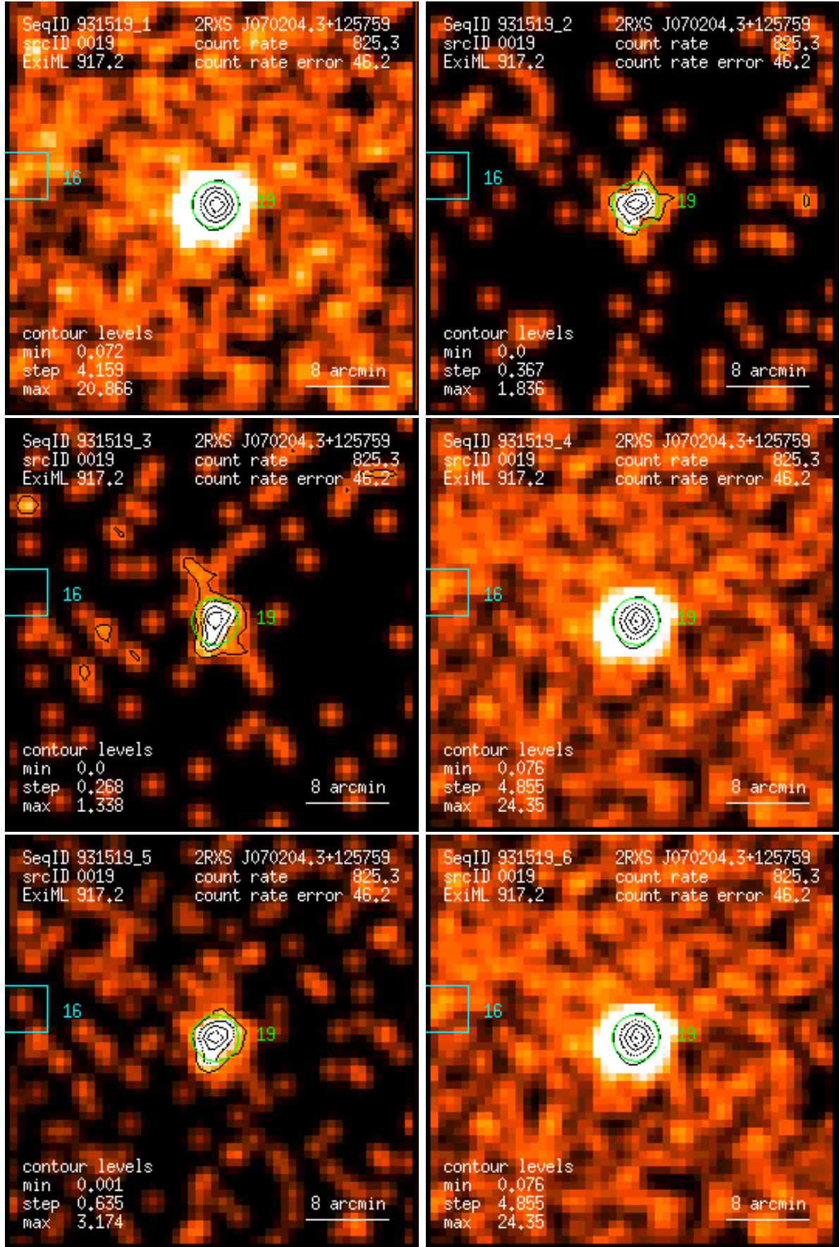
Figure 19: RASS 931519: detection 0019: band rate images, Gaussian filter: (1) PSPC channels 11 – 41, (2) 52 – 90, (3) 91 – 201, (4) 11 – 235, (5) 52 – 201, (6) 11 – 201. Broad band rates in counts/ks. Band rate contour levels in counts/ks/arcmin 2 .
