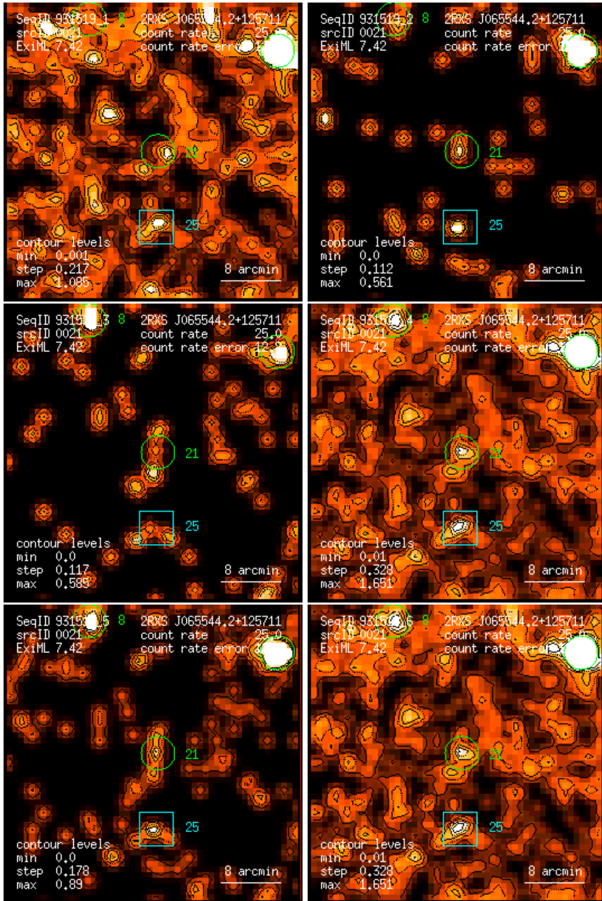
Figure 21: RASS 931519: detection 0021: band rate images, Gaussian filter: (1) PSPC channels 11 – 41, (2) 52 – 90, (3) 91 – 201, (4) 11 – 235, (5) 52 – 201, (6) 11 – 201. Broad band rates in counts/ks. Band rate contour levels in counts/ks/arcmin 2 .
