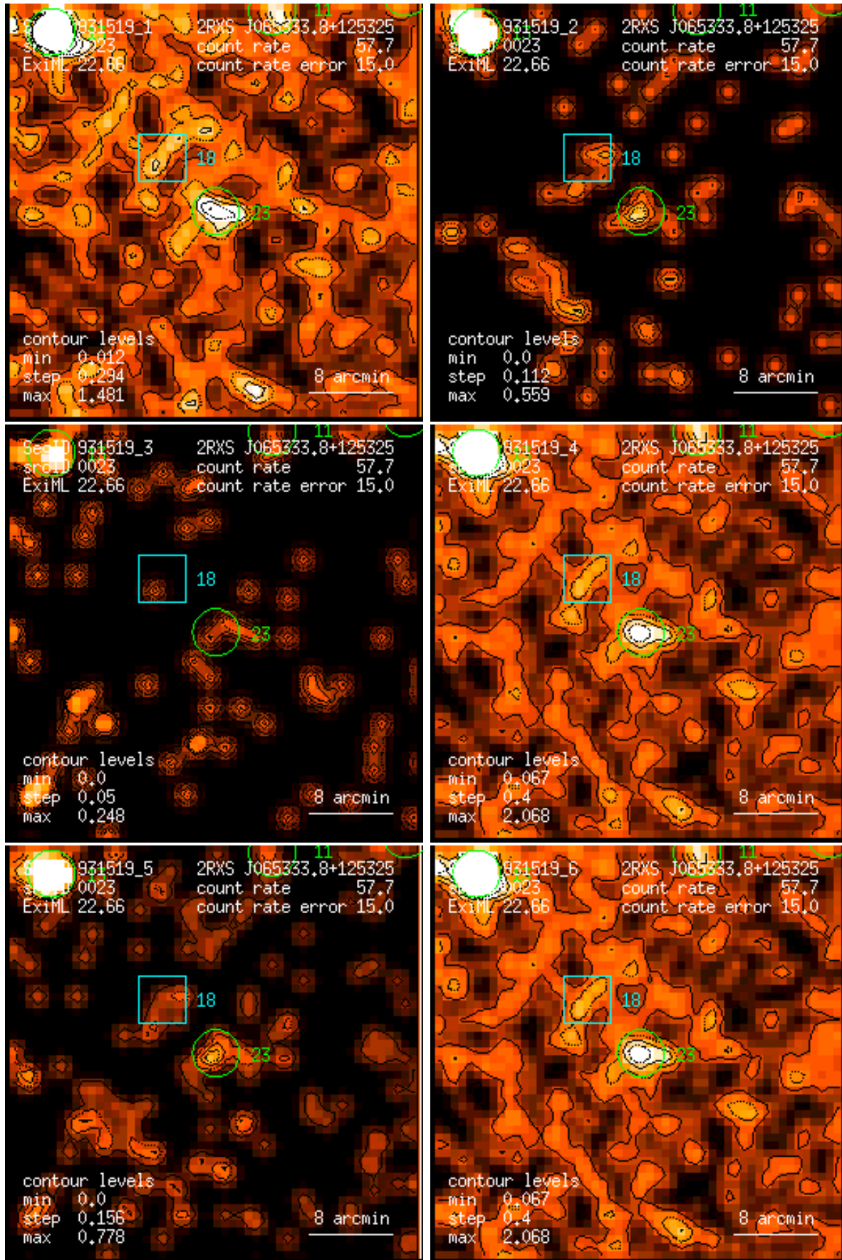
Figure 23: RASS 931519: detection 0023: band rate images, Gaussian filter: (1) PSPC channels 11 – 41, (2) 52 – 90, (3) 91 – 201, (4) 11 – 235, (5) 52 – 201, (6) 11 – 201. Broad band rates in counts/ks. Band rate contour levels in counts/ks/arcmin 2 .
