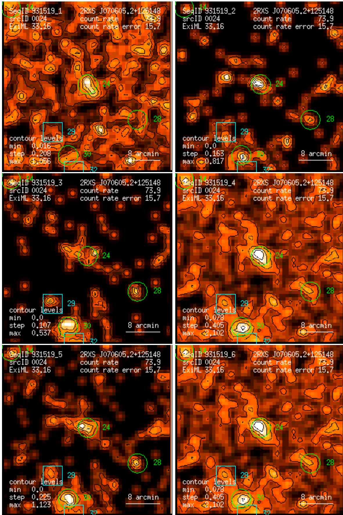
Figure 24: RASS 931519: detection 0024: band rate images, Gaussian filter: (1) PSPC channels 11 – 41, (2) 52 – 90, (3) 91 – 201, (4) 11 – 235, (5) 52 – 201, (6) 11 – 201. Broad band rates in counts/ks. Band rate contour levels in counts/ks/arcmin 2 .
