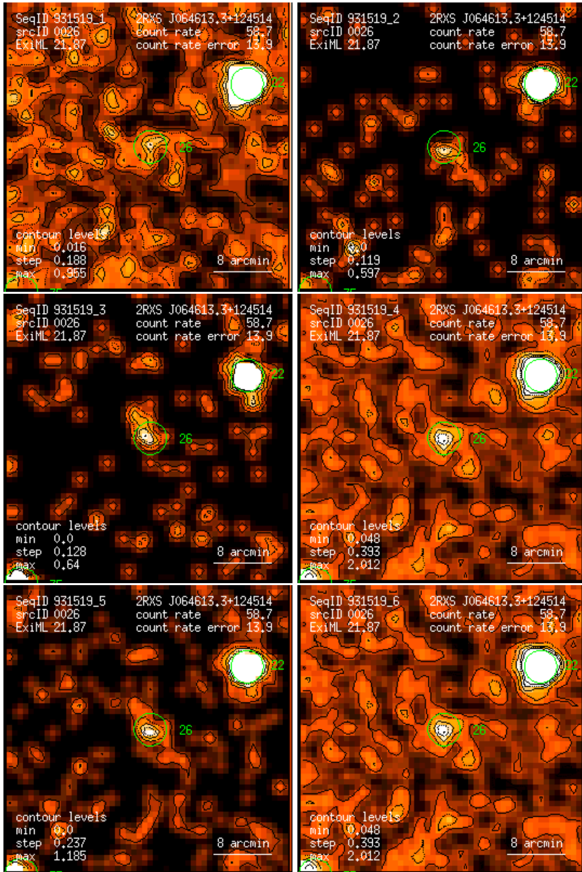
Figure 26: RASS 931519: detection 0026: band rate images, Gaussian filter: (1) PSPC channels 11 – 41, (2) 52 – 90, (3) 91 – 201, (4) 11 – 235, (5) 52 – 201, (6) 11 – 201. Broad band rates in counts/ks. Band rate contour levels in counts/ks/arcmin 2 .
