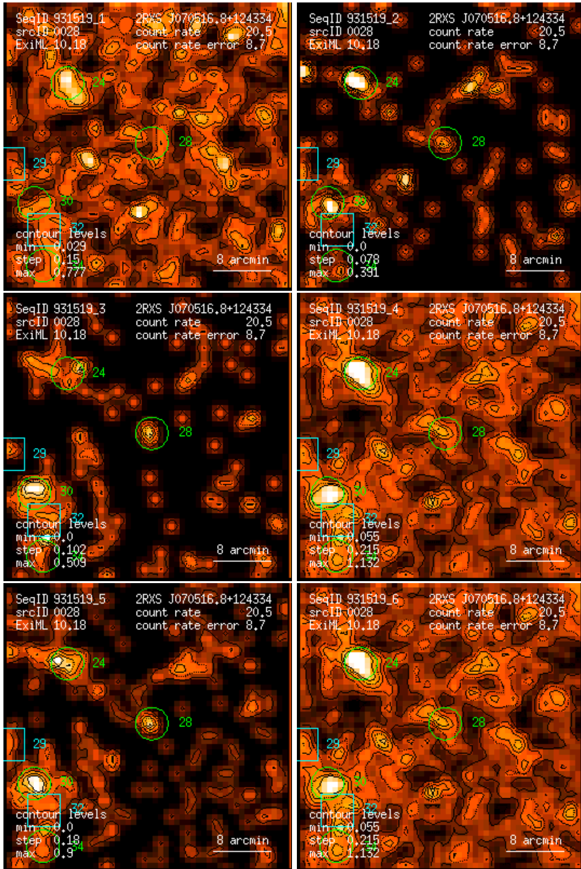
Figure 28: RASS 931519: detection 0028: band rate images, Gaussian filter: (1) PSPC channels 11 – 41, (2) 52 – 90, (3) 91 – 201, (4) 11 – 235, (5) 52 – 201, (6) 11 – 201. Broad band rates in counts/ks. Band rate contour levels in counts/ks/arcmin 2 .
