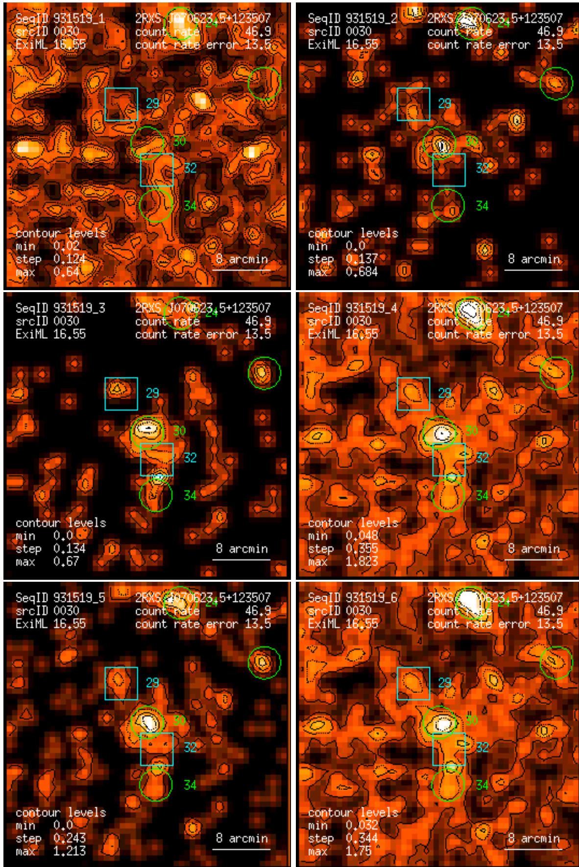
Figure 30: RASS 931519: detection 0030: band rate images, Gaussian filter: (1) PSPC channels 11 – 41, (2) 52 – 90, (3) 91 – 201, (4) 11 – 235, (5) 52 – 201, (6) 11 – 201. Broad band rates in counts/ks. Band rate contour levels in counts/ks/arcmin 2 .
