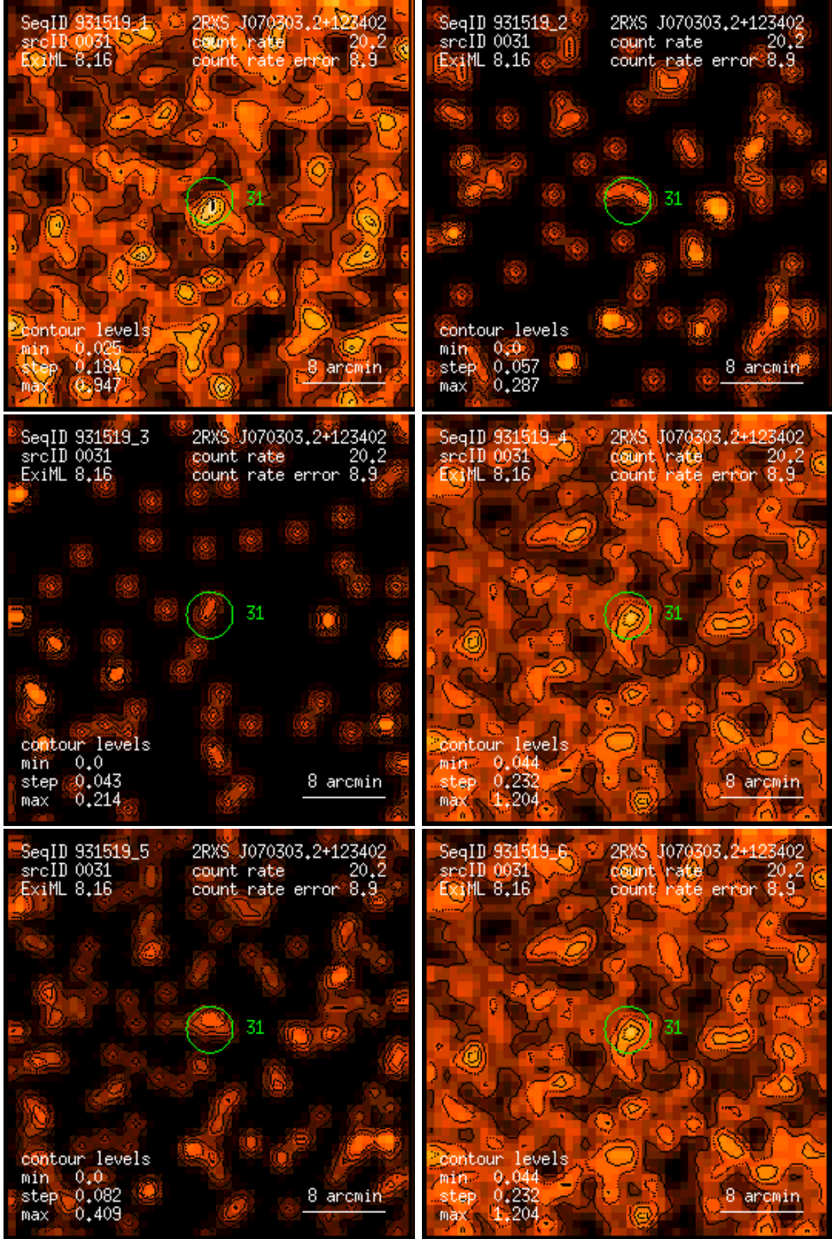
Figure 31: RASS 931519: detection 0031: band rate images, Gaussian filter: (1) PSPC channels 11 – 41, (2) 52 – 90, (3) 91 – 201, (4) 11 – 235, (5) 52 – 201, (6) 11 – 201. Broad band rates in counts/ks. Band rate contour levels in counts/ks/arcmin 2 .
